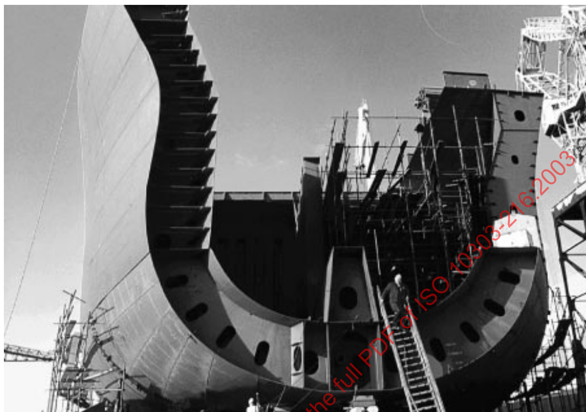
Figure 20 — Double ship hull
