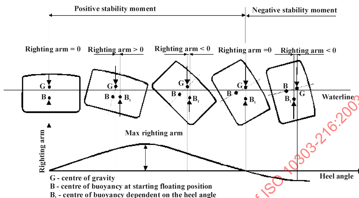
Figure 50 — Form stability
