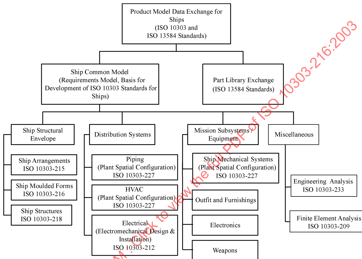
Figure 1 — Shipbuilding application protocols
