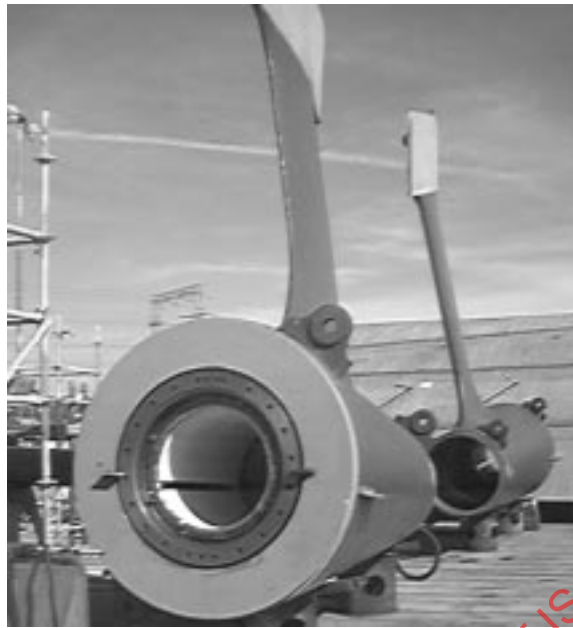
Figure 7 — Shaft struts
