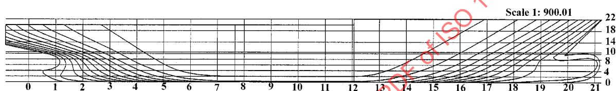
Figure 39 — Buttock lines
