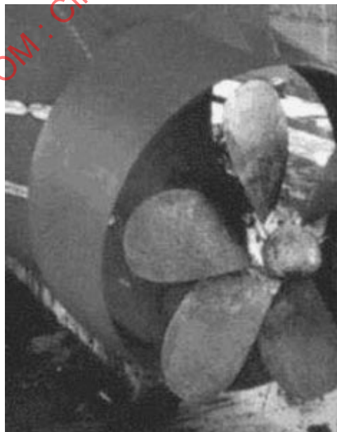
Figure 35 — Ducted propeller
