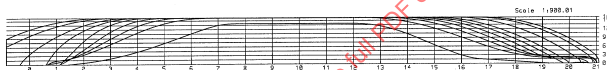
Figure 41 — Waterlines
