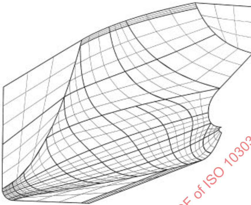
Figure 38 — Ship curves
