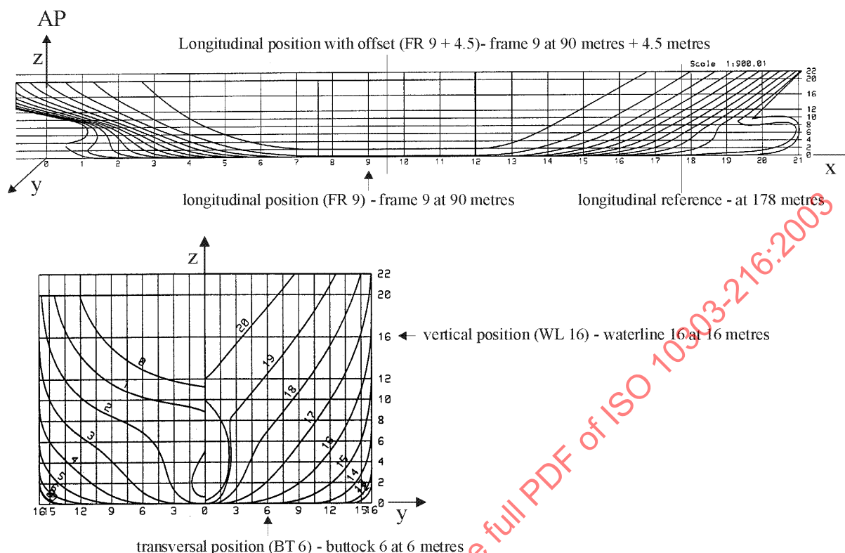
Figure 47 — Spacing position
