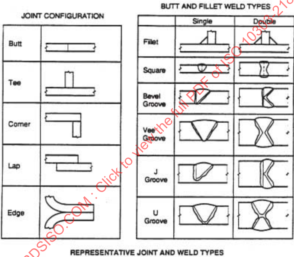
Figure 65 — Weld types
