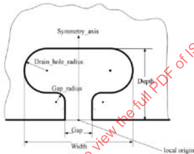
Figure 17 — Drain_hole_cutout
