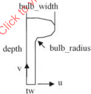
Figure 7 — Bulbflat_cross_section
