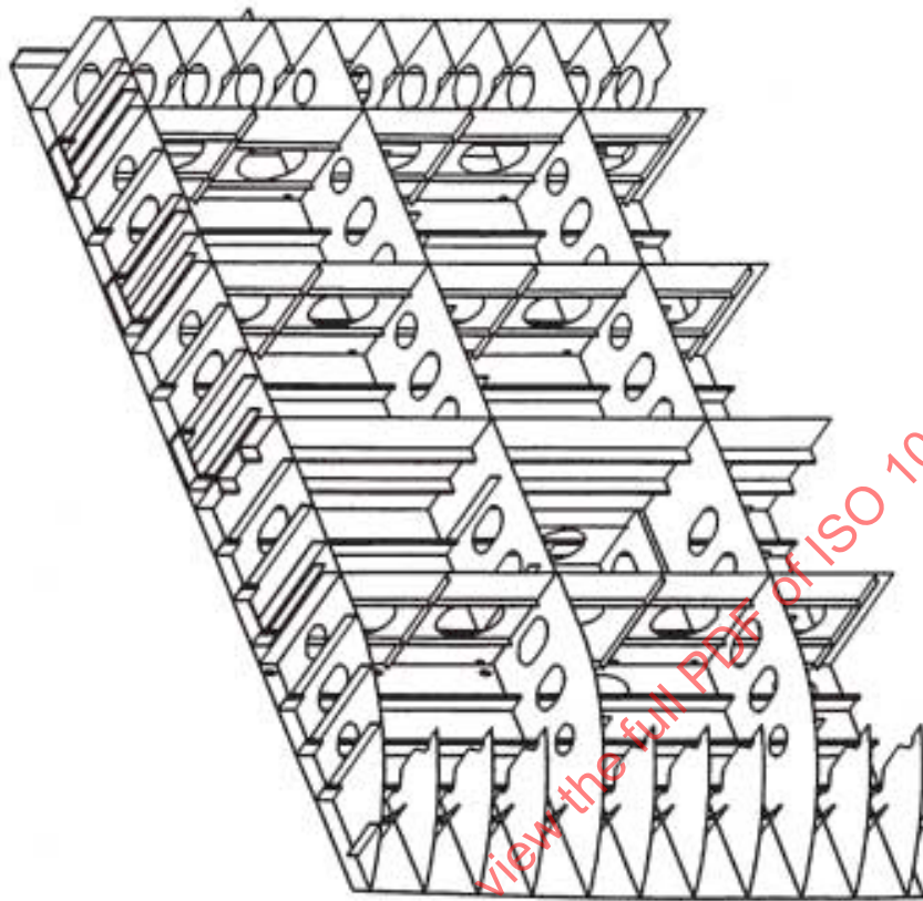
Figure 4 — Assembly
