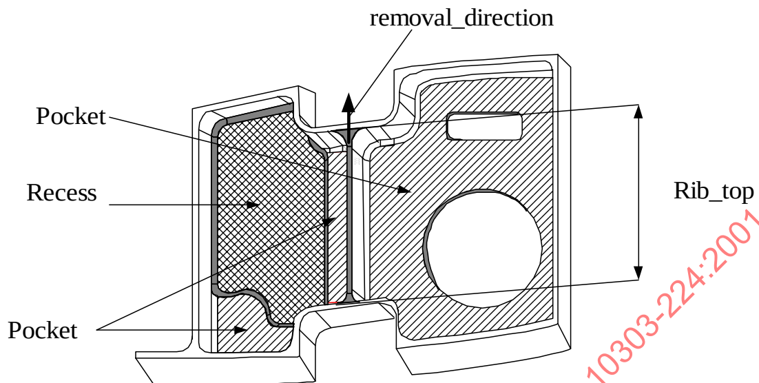
Figure 90 - Rib_top
