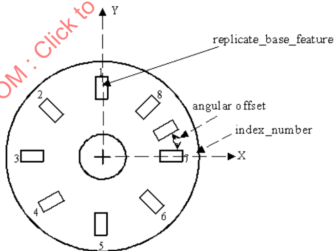
Figure 16 - Circular_offset_pattern
