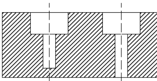
Figure 28 - Counterbore_hole
