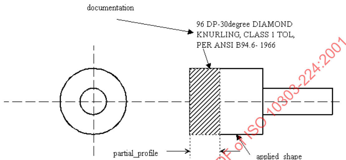
Figure 9 - Catalogue_knurl
