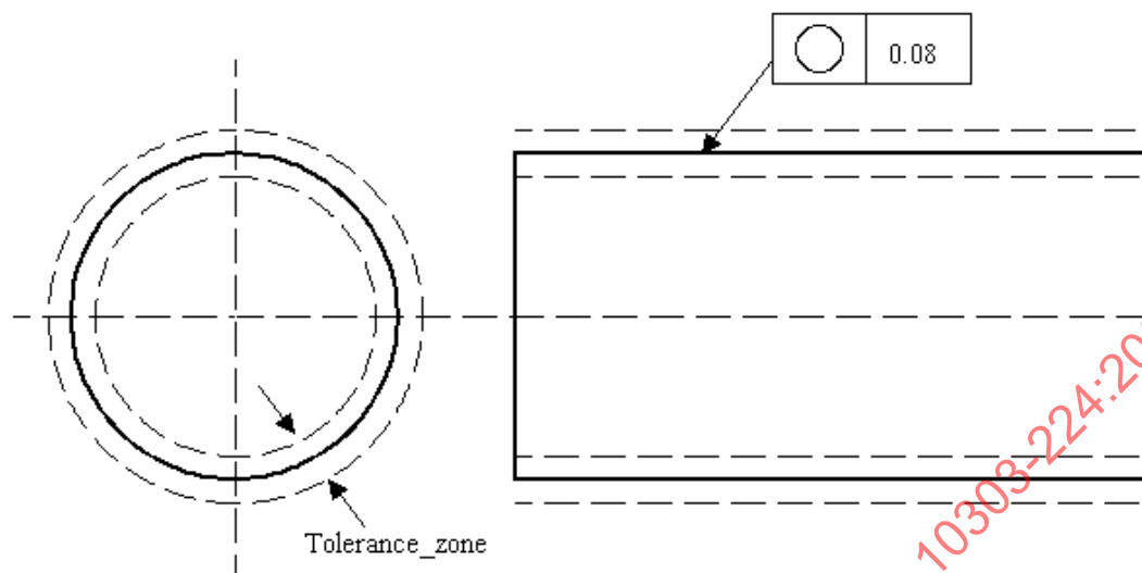
Figure 21 - Circularity_tolerance
