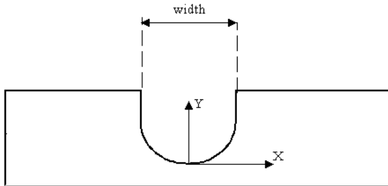
Figure 93 - Rounded_U_profile
