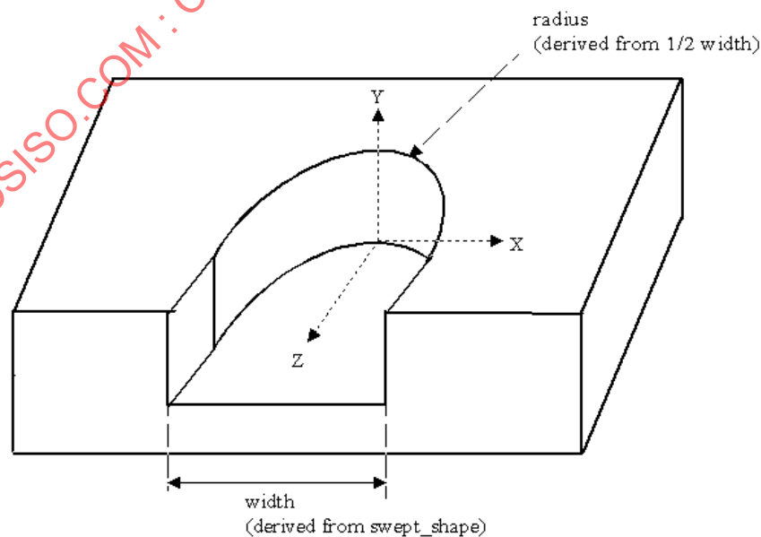
Figure 79 - Radiused_slot_end_type
