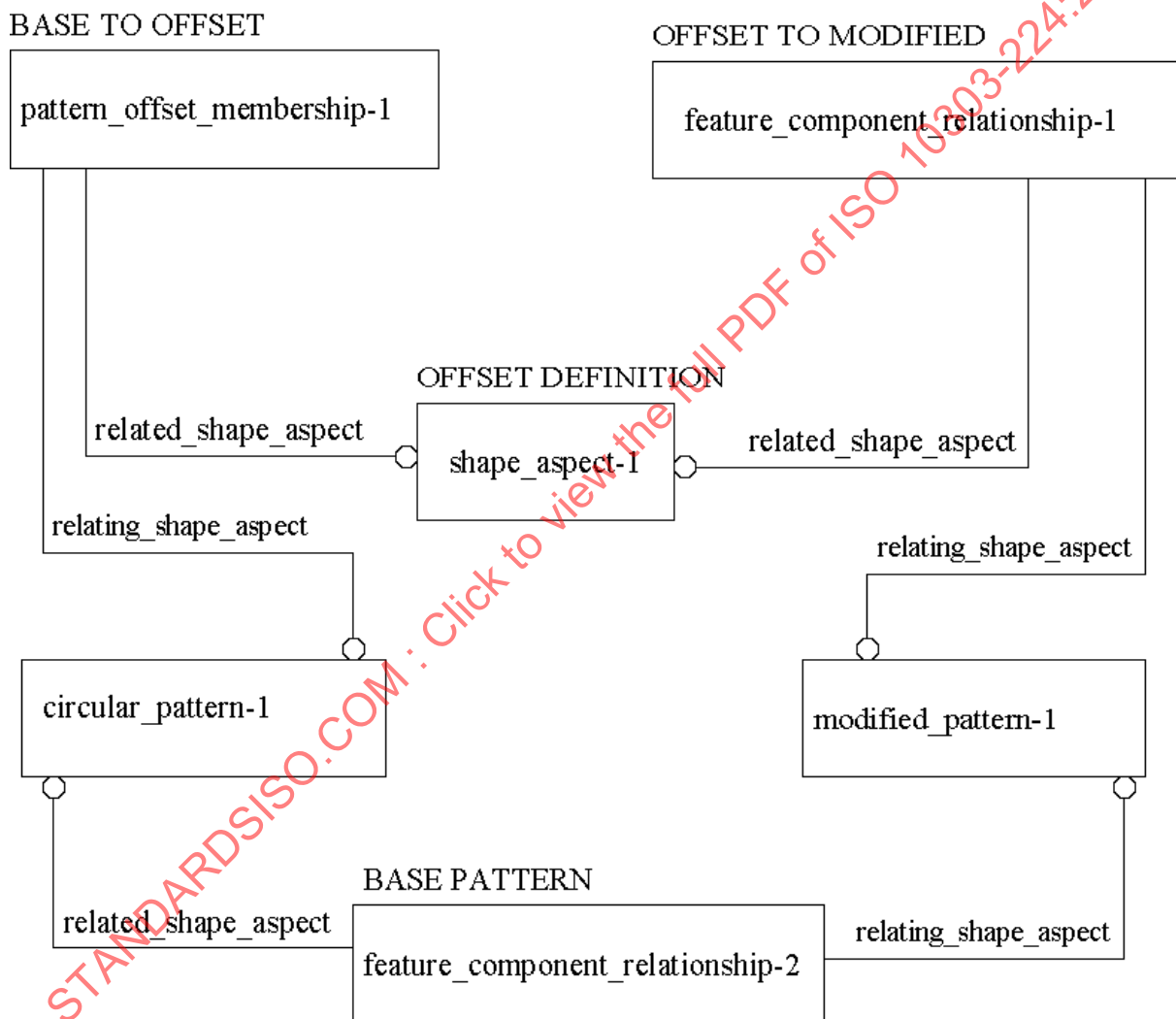
Figure 111 - Pattern offset required instances
