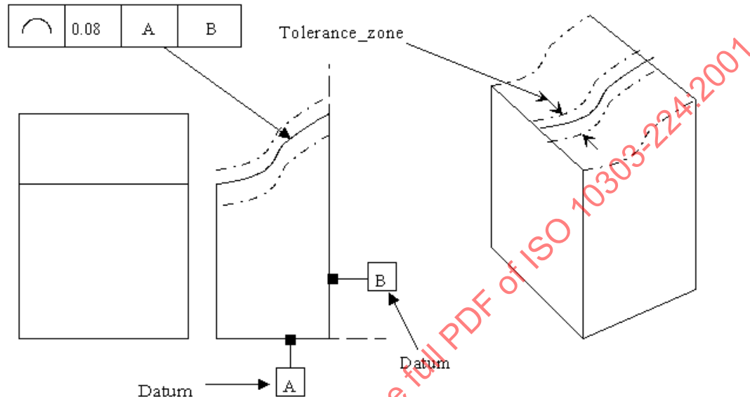
Figure 61 - Linear_profile_tolerance
