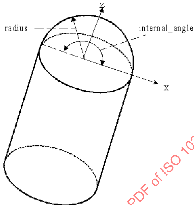
Figure 96 - Spherical_cap
