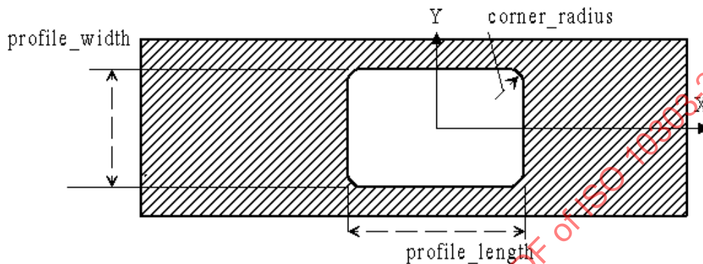
Figure 83 - Rectangular_closed_profile
