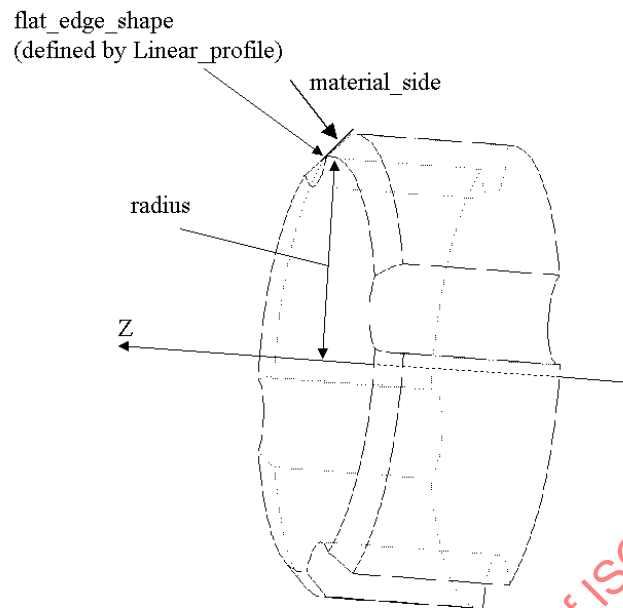
Figure 88 - Revolved flat
