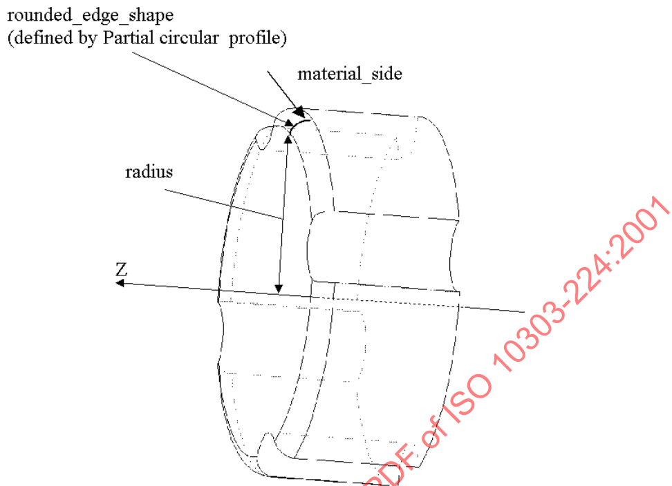
Figure 89 - Revolved_round
