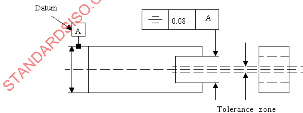
Figure 103 - Symmetry_tolerance
