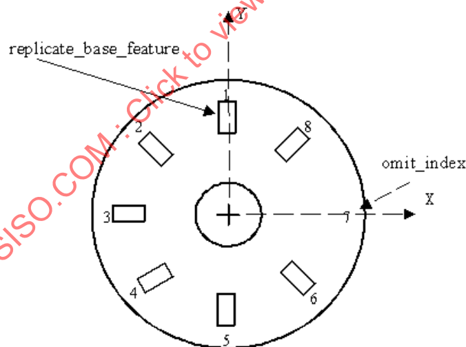
Figure 17 - Circular_omit_pattern
