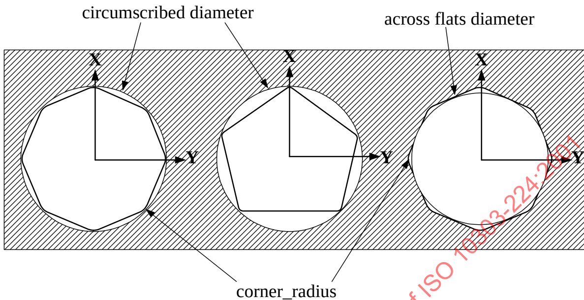
Figure 65 - Ngon_profile
