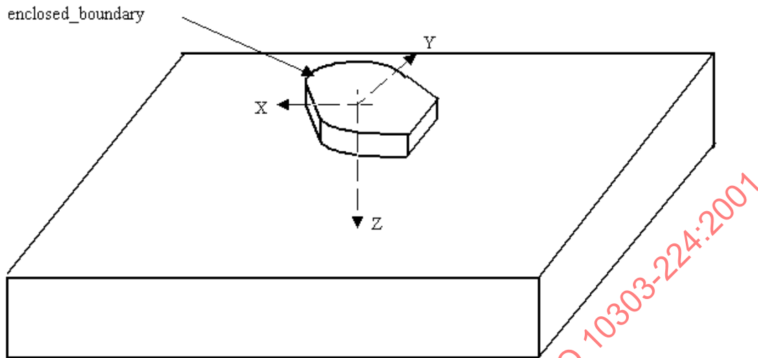
Figure 46 - General_boss
