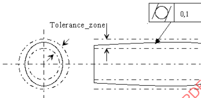
Figure 33 - Cylindricity_tolerance
