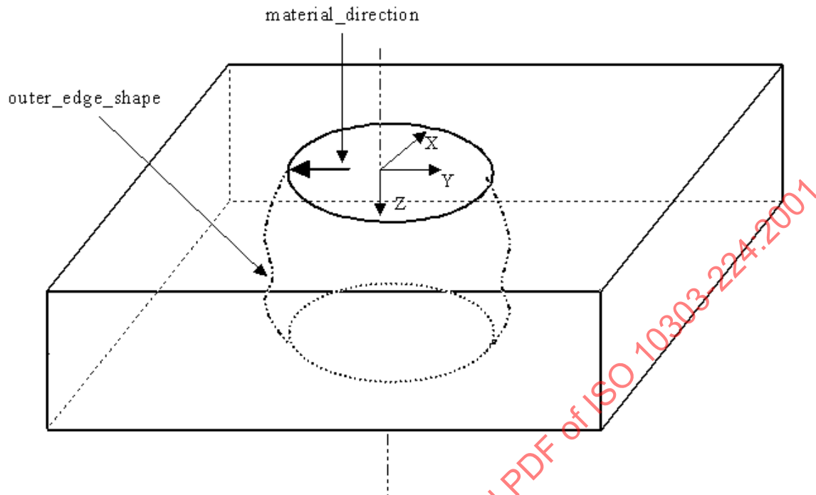
Figure 55 - General_revolution for volume removal
