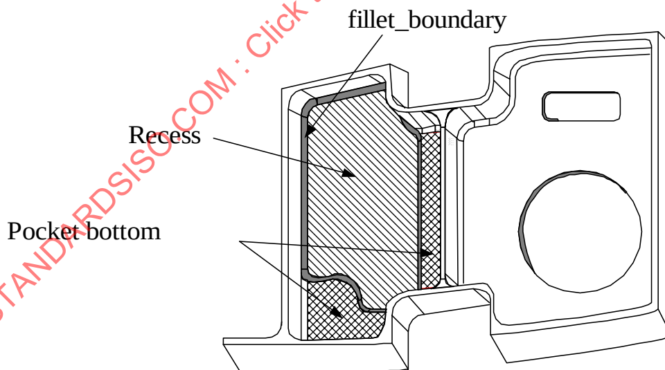
Figure 80 - Recess
