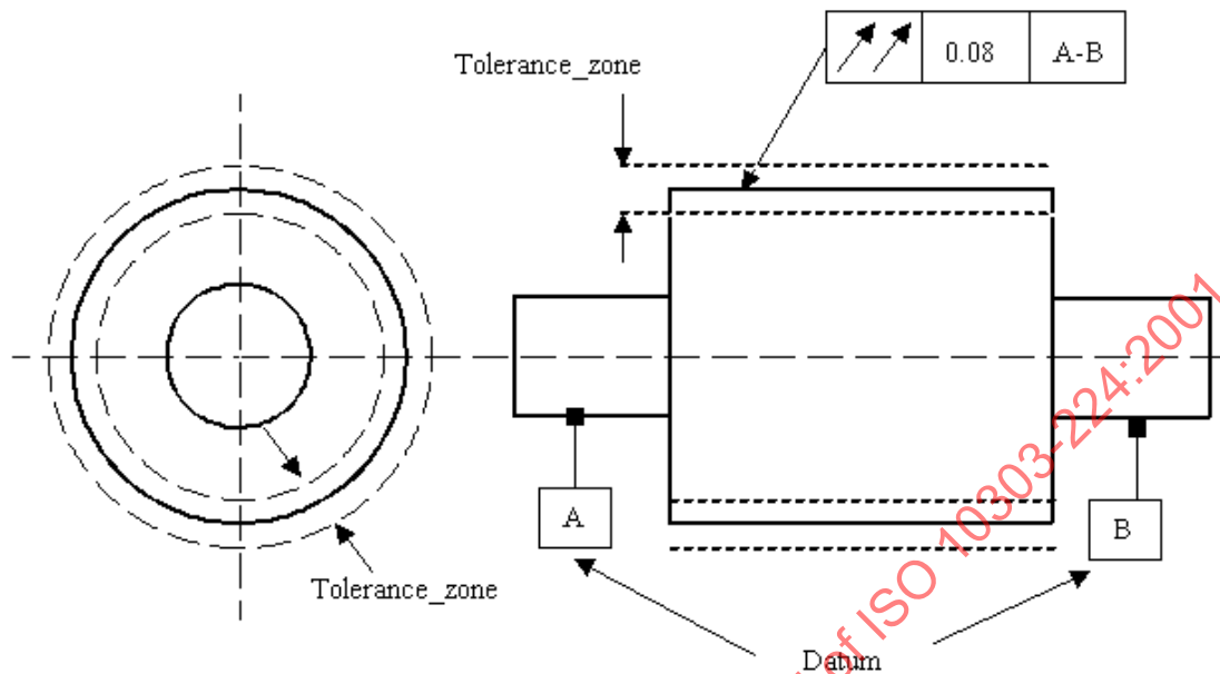
Figure 107 - Total_runout_tolerance
