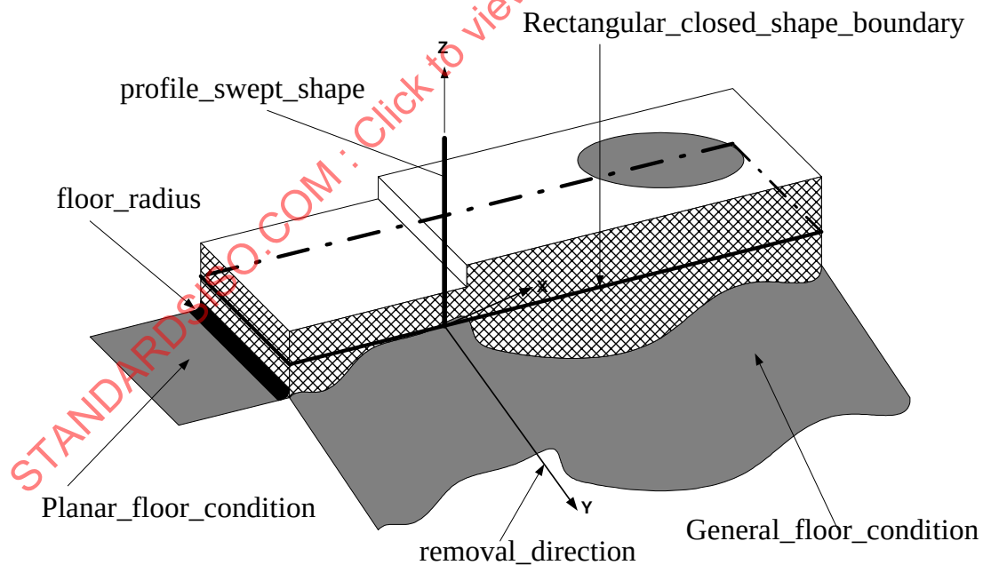
Figure 94 - Shape_profile
