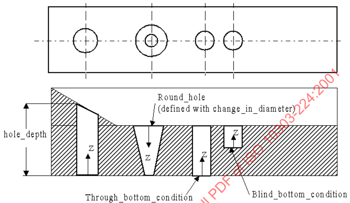
Figure 91 - Round_hole
