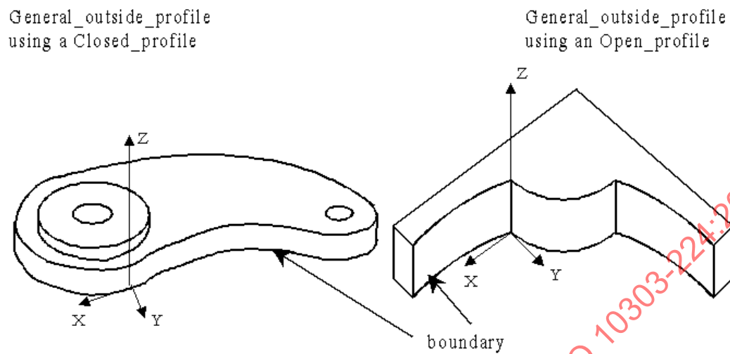
Figure 49 - General_outside_profile
