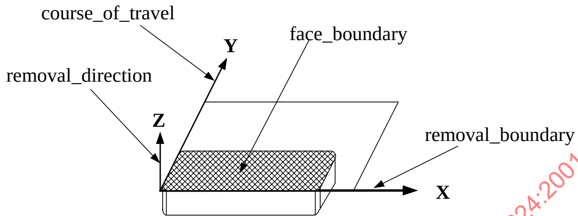
Figure 74 - Planar_face
