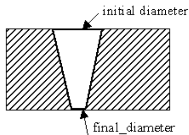
Figure 38 - Diameter_taper
