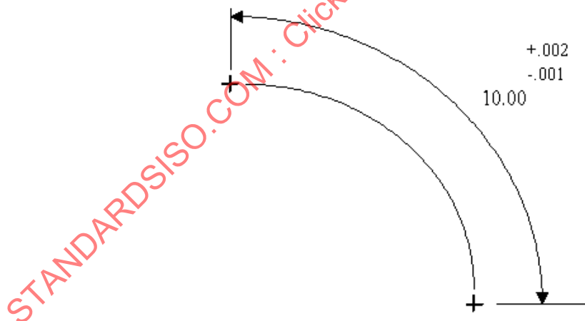
Figure 40 - Distance_along_curve_tolerance
