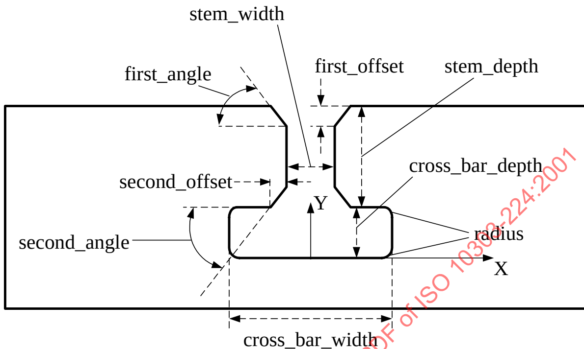
Figure 104 - Tee_profile
