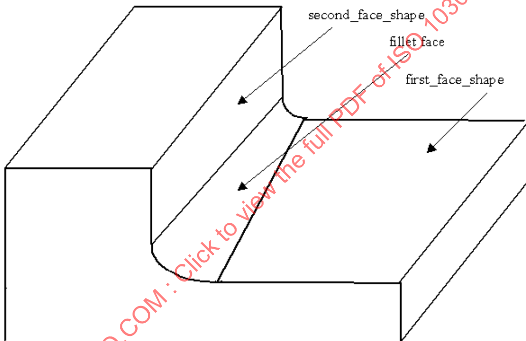
Figure 42 - Fillet
