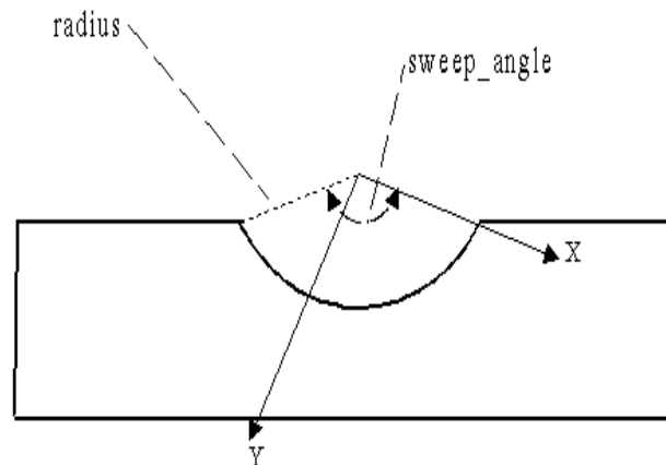
Figure 72 - Partial_circular_profile
