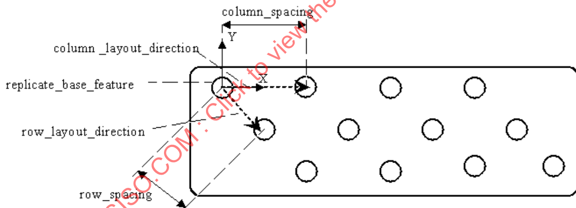
Figure 87 - Rectangular_pattern
