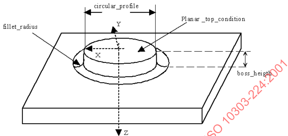
Figure 13 - Circular_boss
