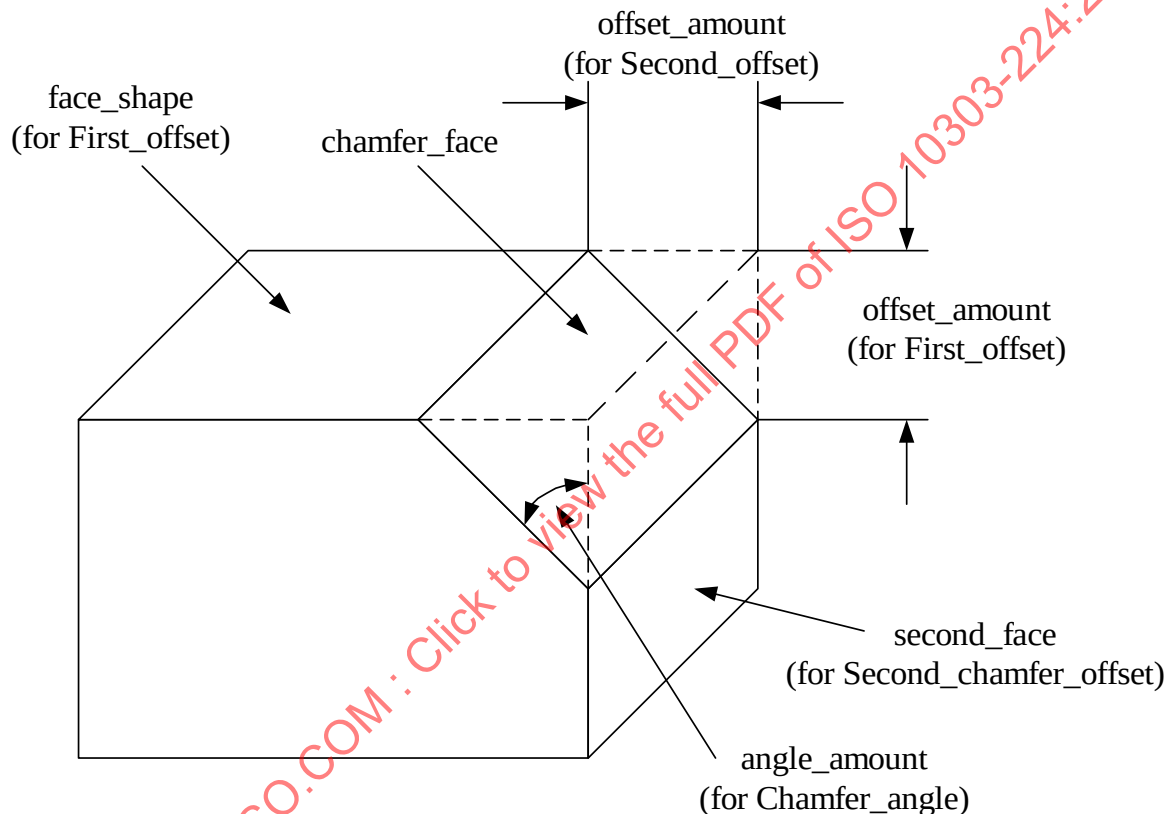
Figure 12 - Chamfer
