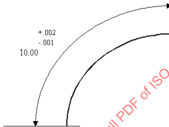
Figure 33 — Curved_dimension_tolerance
