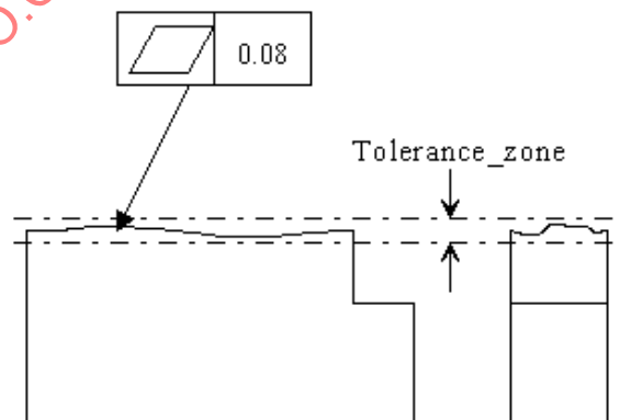
Figure 48 — Flatness_tolerance
