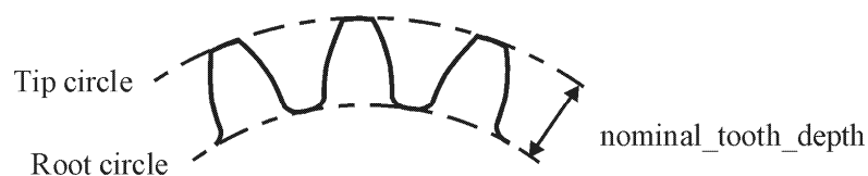
Figure 50 — Gear nominal_tooth_depth
