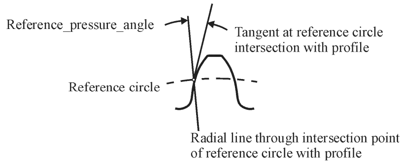
Figure 52 — Gear reference_pressure_angle
