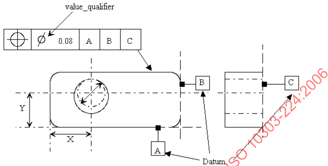
Figure 89 — Position_tolerance
