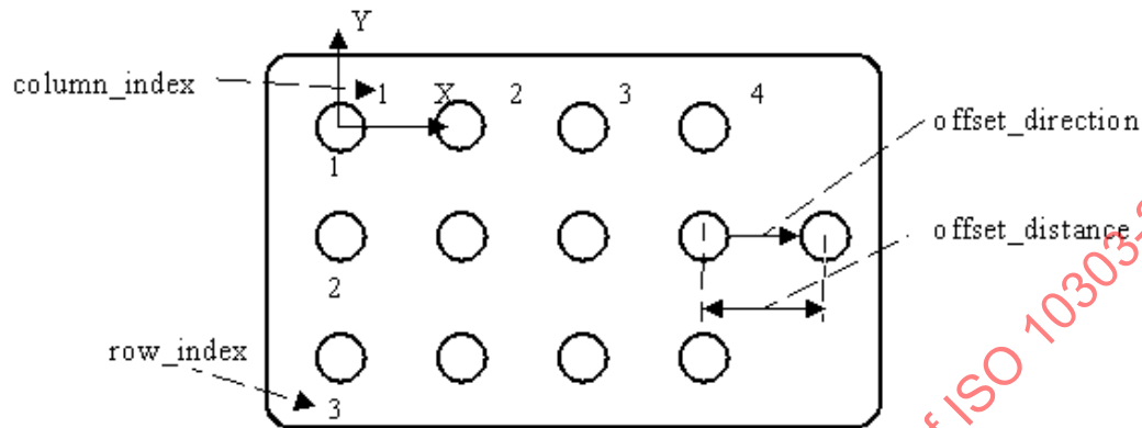
Figure 97 — Rectangular_offset_pattern
