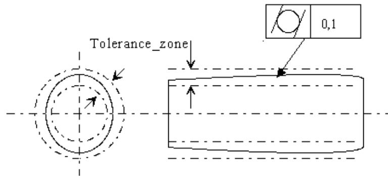
Figure 36 — Cylindricity_tolerance
