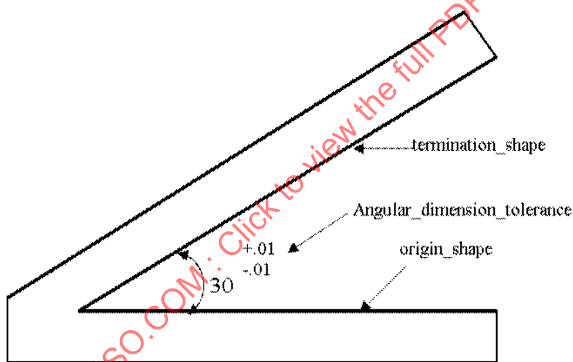
Figure 3 — Angular_dimension_tolerance
