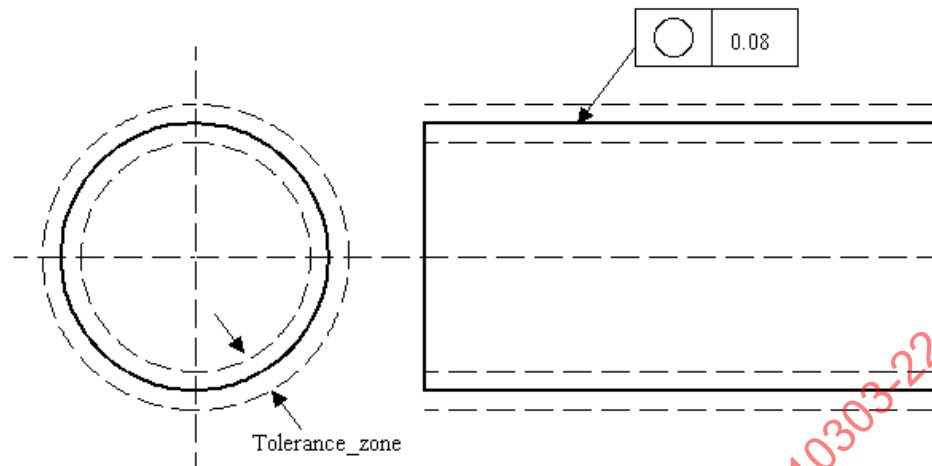
Figure 24 — Circularity_tolerance
