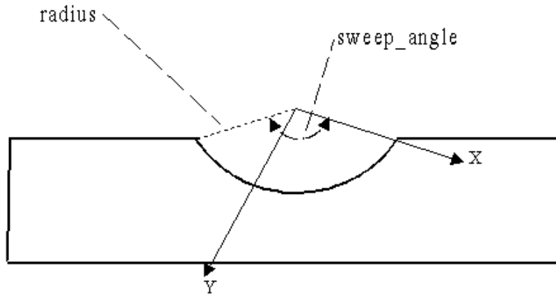
Figure 84 — Partial_circular_profile
