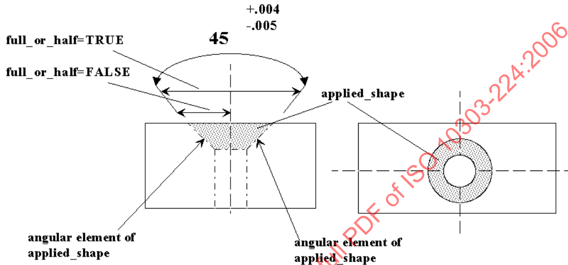
Figure 4 — Angular_size_dimension_tolerance
