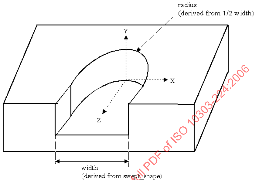
Figure 92 — Radiused_slot_end_type
