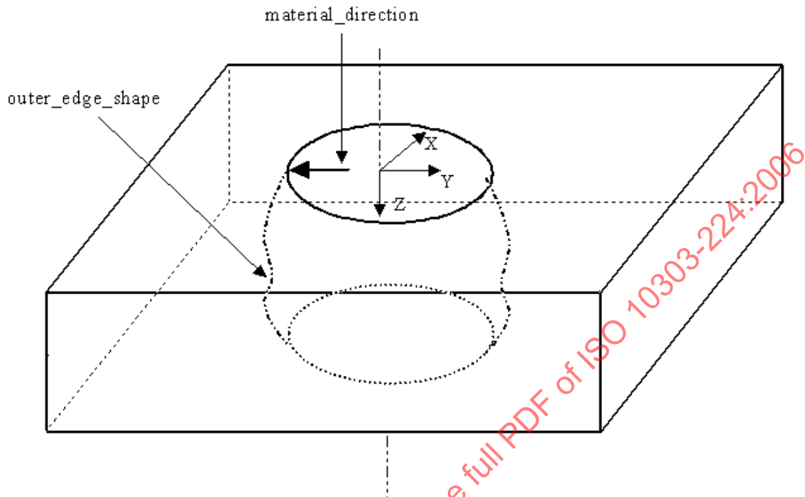
Figure 64 — General_revolution for a volume removal
