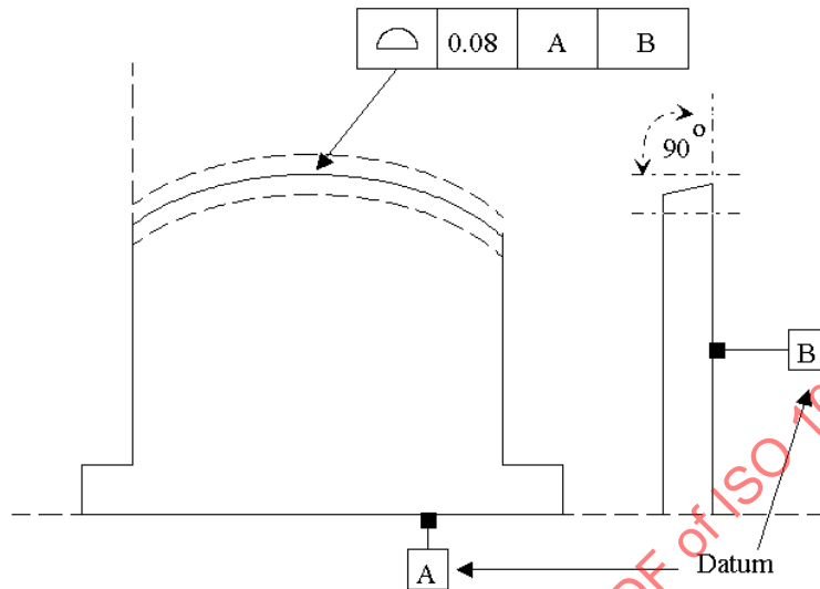
Figure 116 — Surface_profile_tolerance
