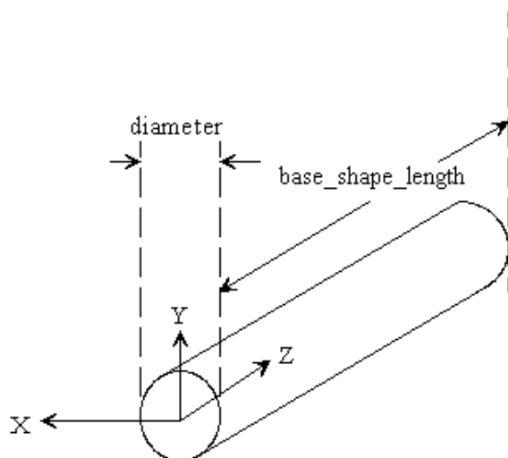
Figure 35 — Cylindrical_base_shape
