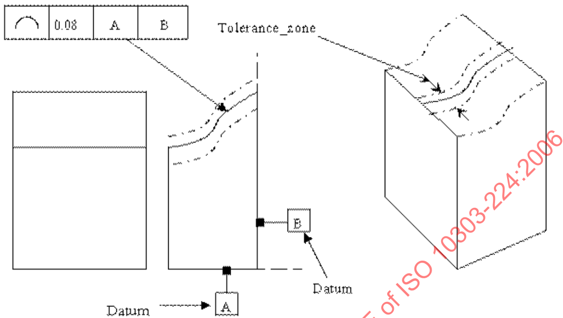
Figure 73 — Linear_profile_tolerance
