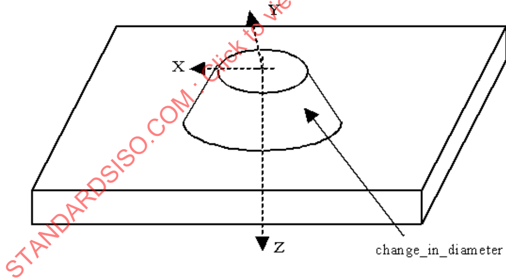
Figure 17 — Circular_boss with taper
