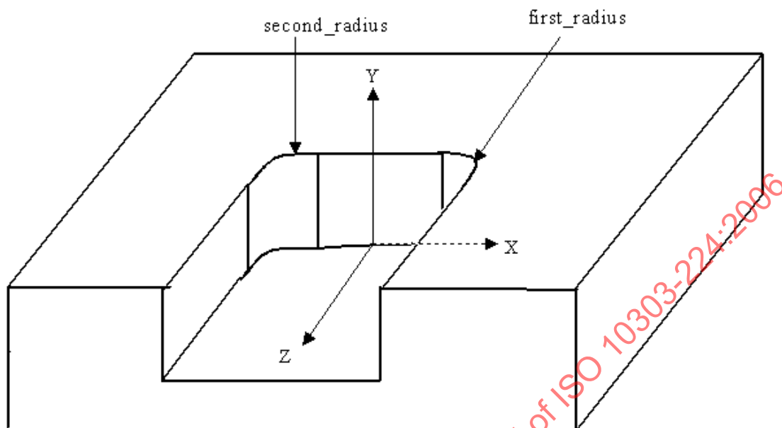
Figure 47 — Flat_slot_end_type
