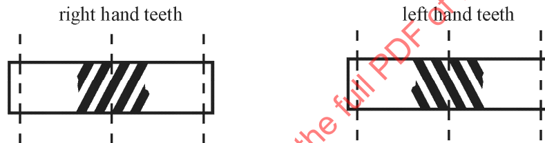
Figure 67 — Helical_gear left_or_right_hand_tooth
