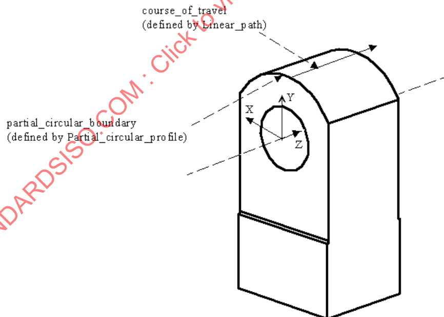
Figure 105 — Rounded_end
