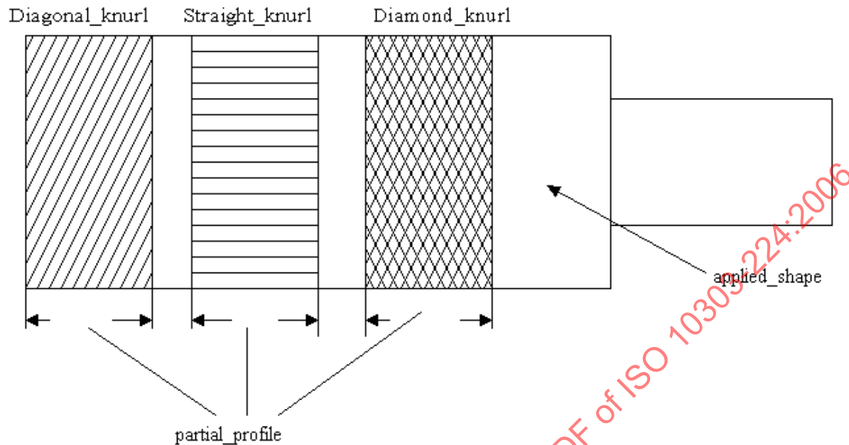
Figure 70 — Knurl
