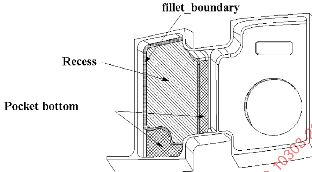
Figure 93 — Recess
