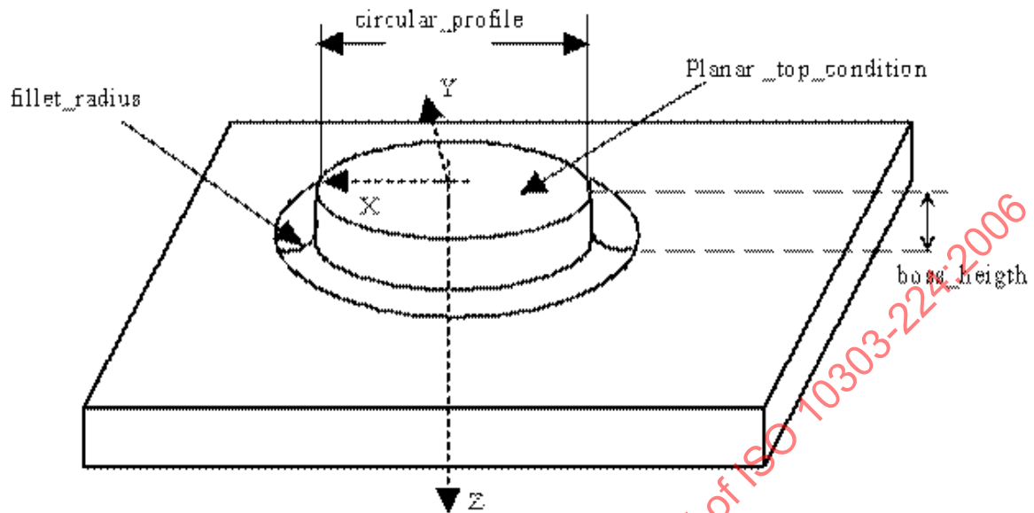
Figure 16 — Circular_boss
