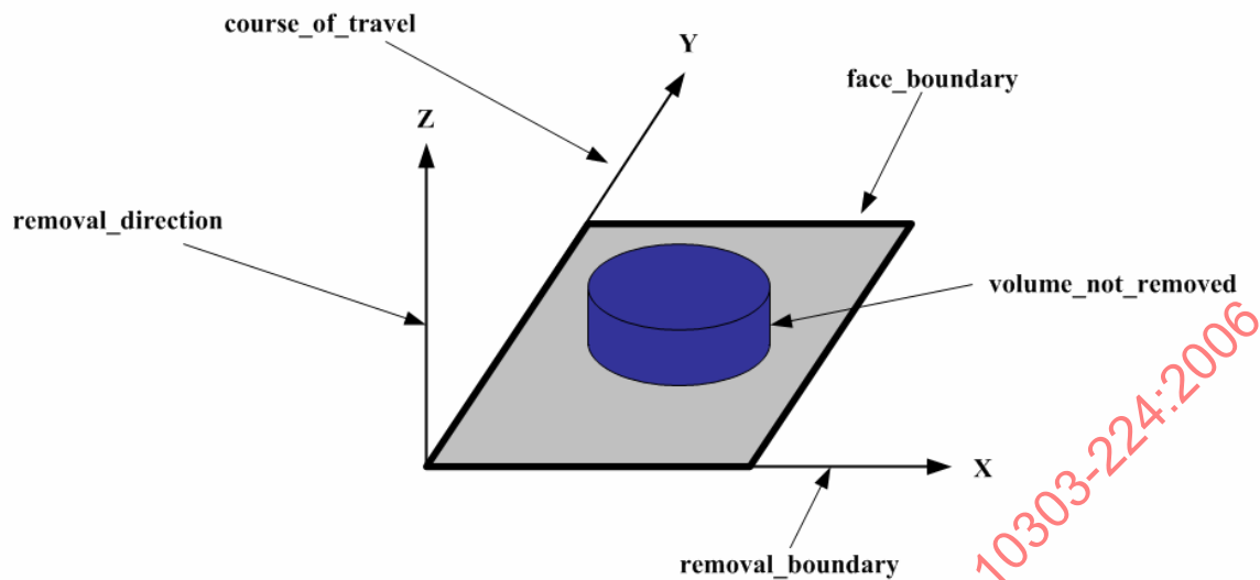
Figure 87 — Planar_face
