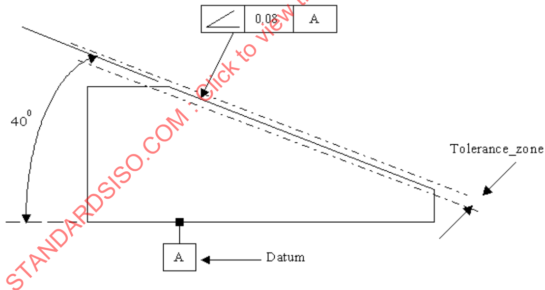
Figure 5 — Angularity_tolerance for a plane surface
