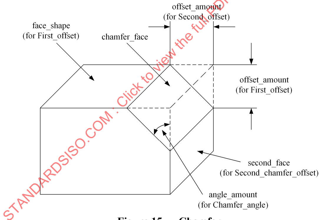
Figure 15 — Chamfer
