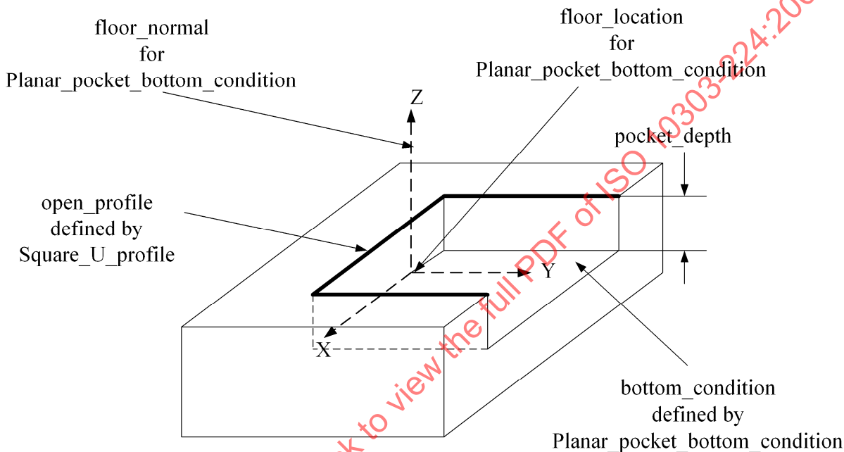
Figure 99 — Rectangular_open_pocket
