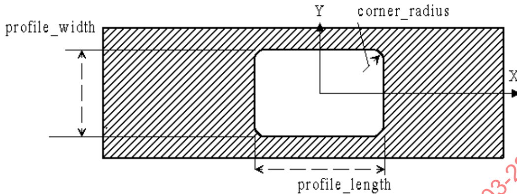
Figure 96 — Rectangular_closed_profile
