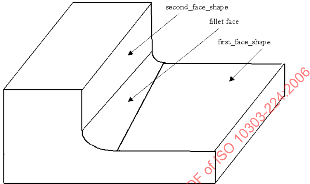
Figure 45 — Fillet
