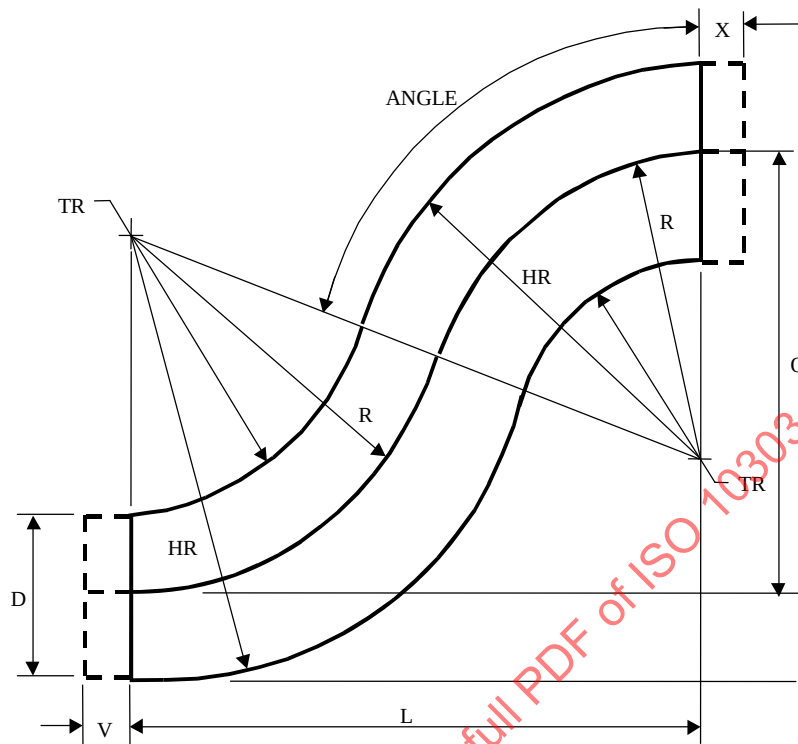
Figure 36 — Hvac_offset_ogee_centred
