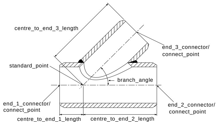
Figure 42 — Lateral
