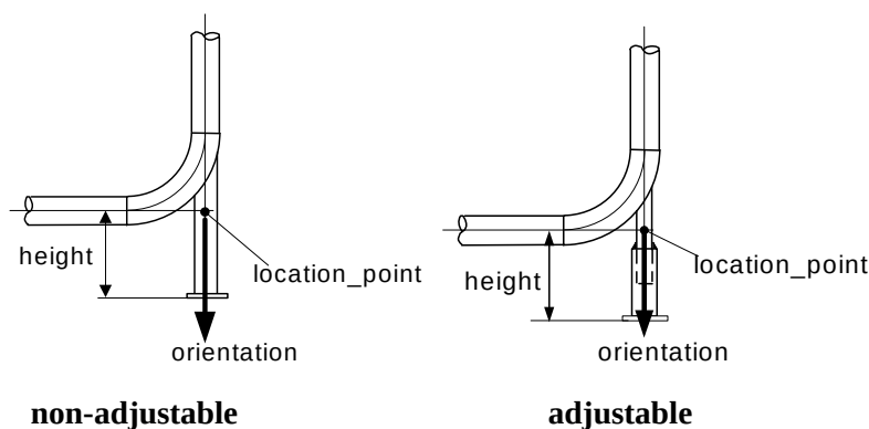
Figure 3 — Base_elbow_support
