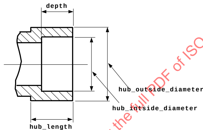
Figure 21 — Female_end
