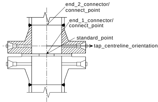
Figure 47 — Orifice_flange
