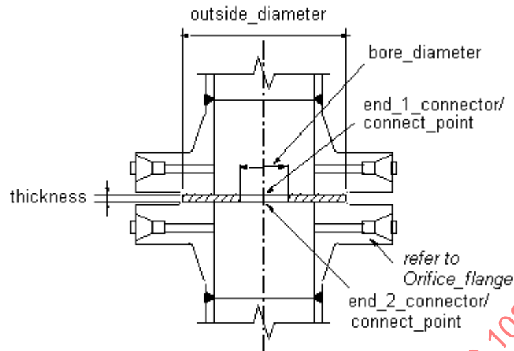
Figure 48 — Orifice_plate
