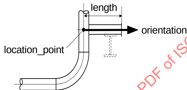
Figure 74 — Trunnion
