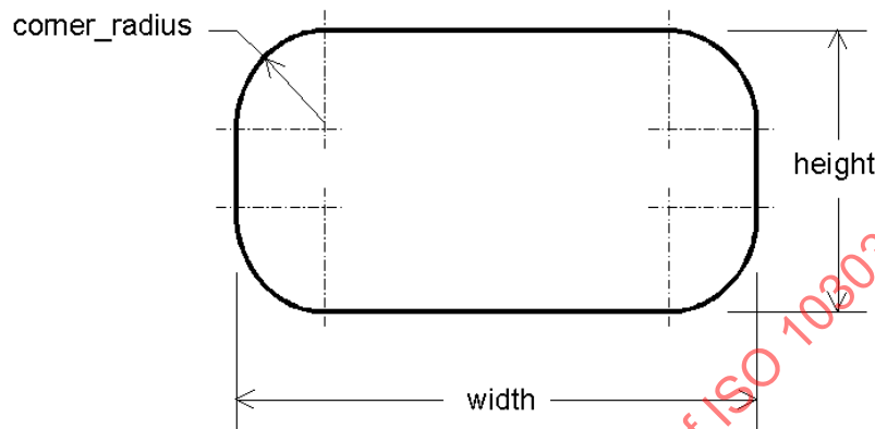
Figure 15 — Cross_section_radiused_corner
