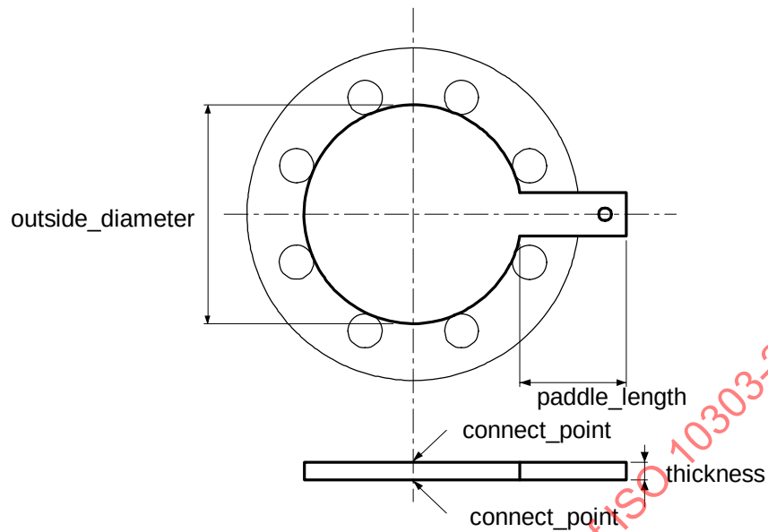
Figure 50 — Paddle_blank
