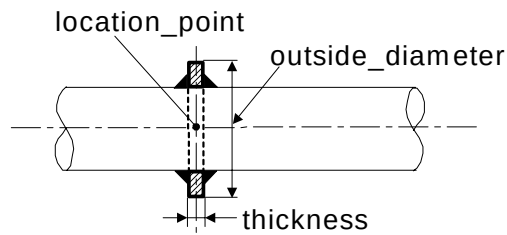
Figure 59 — Reinforcing_ring
