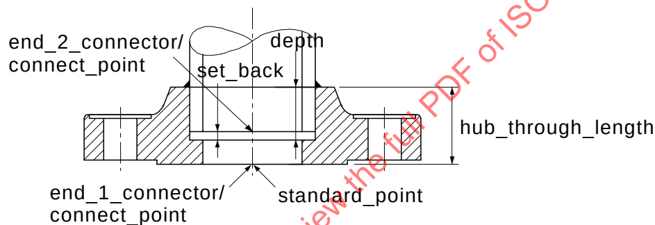
Figure 66 — Socket_weld_flange
