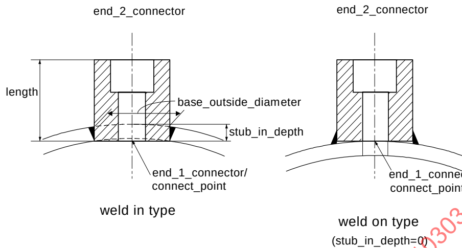
Figure 7 — Boss
