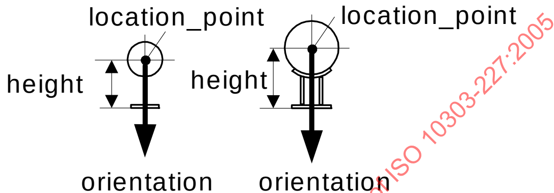
Figure 62 — Shoe
