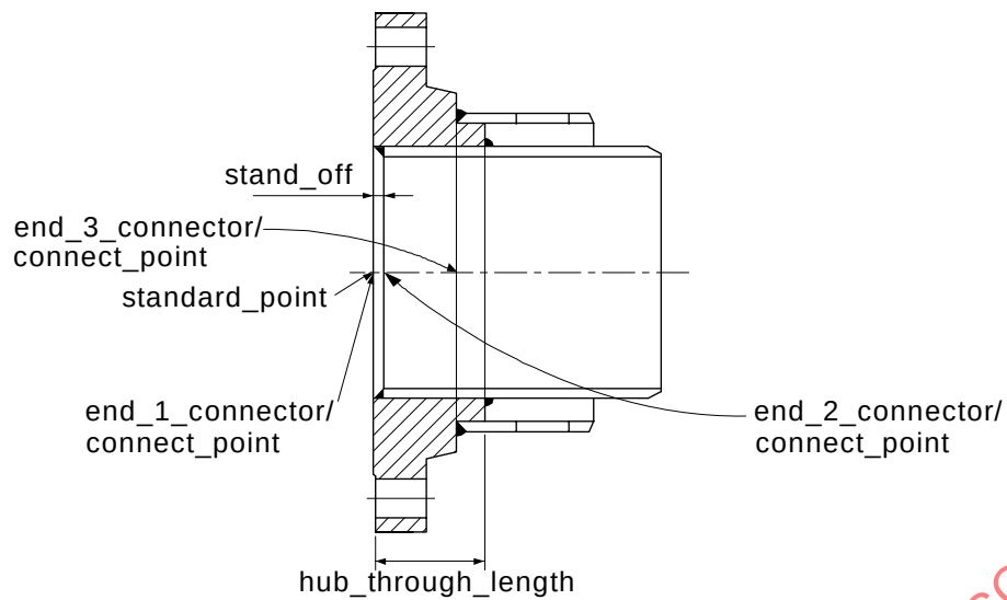
Figure 64 — Slip_on_jacket_flange
