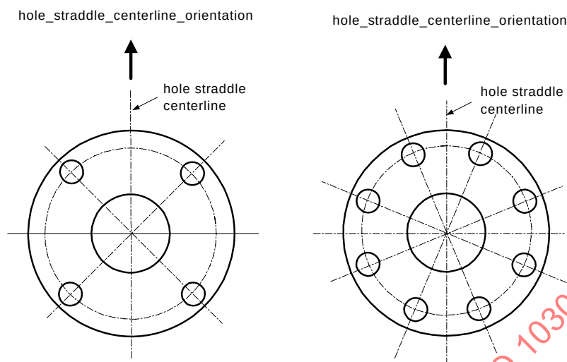
Figure 23 — Hole_straddle_centreline_orientation
