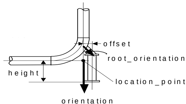
Figure 17 — Eccentric_base_elbow_support
