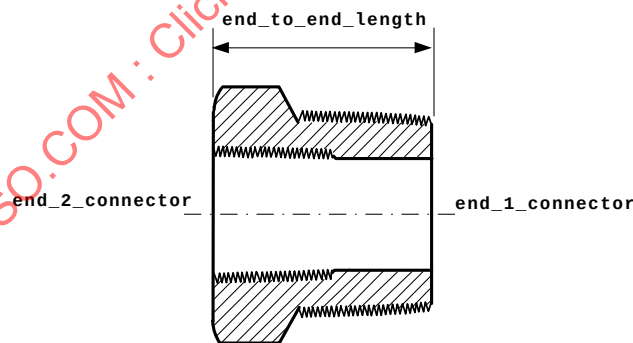
Figure 8 — Bushing
