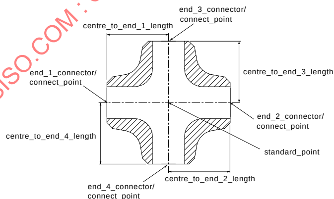
Figure 13 — Butt-weld cross
