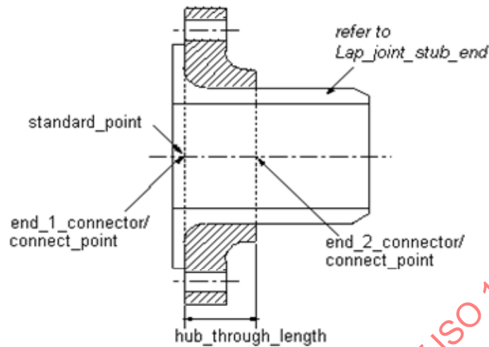
Figure 40 — Lap_joint_flange
