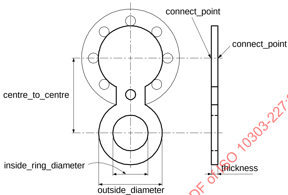
Figure 67 — Spectacle_blind
