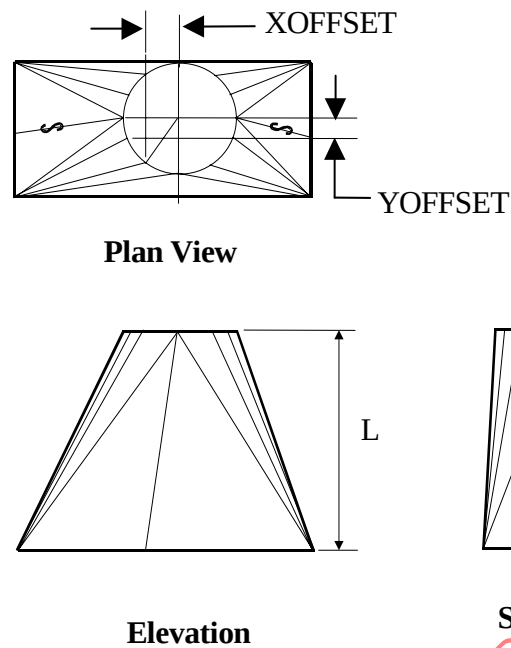
Figure 37 — Transition - rectangular to round
