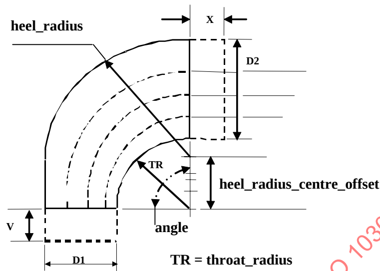
Figure 33 — Hvac_elbow_90deg_reducing
