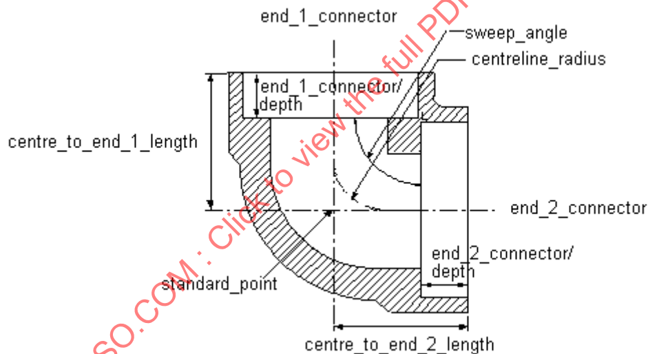
Figure 19 — Elbow
