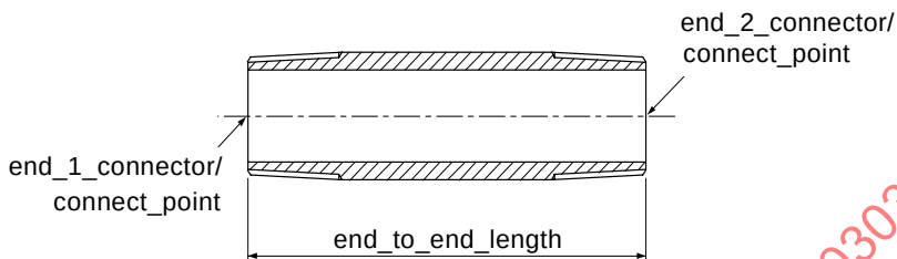
Figure 45 — Nipple
