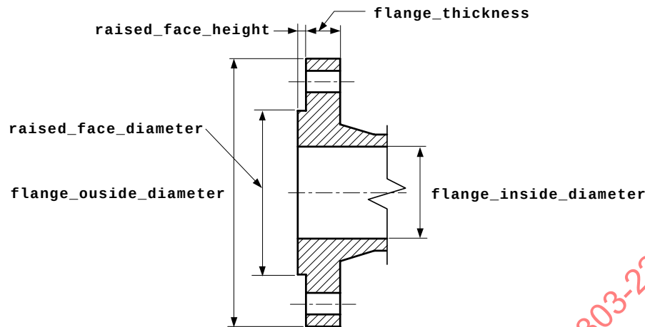
Figure 24 — Flanged_end
