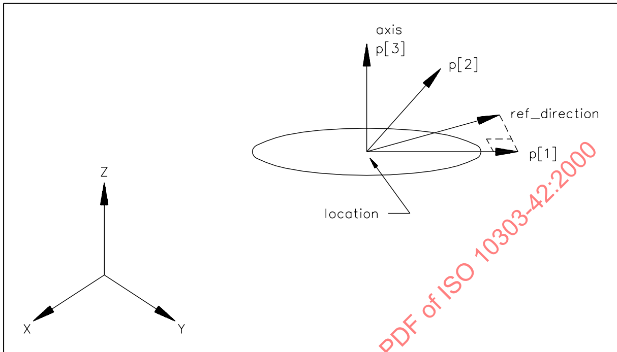
Figure 5 – Ellipse
