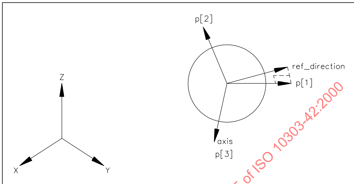
Figure 4 – Circle
