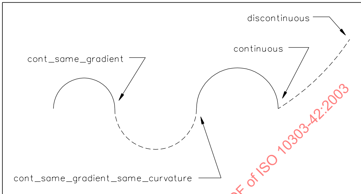
Figure 11 – Composite_curve
