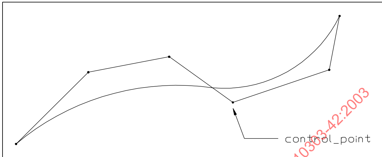
Figure 10 – B-spline curve
