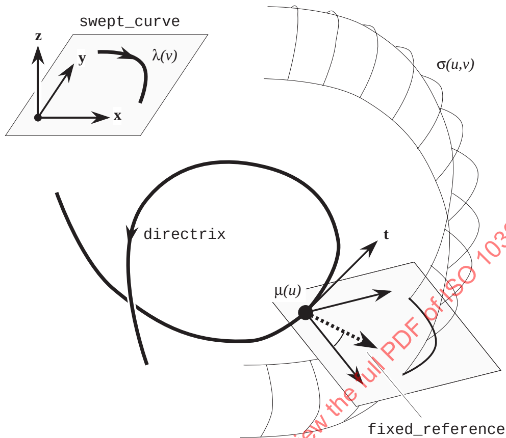
Figure 18 – Fixed_reference_swept_surface
