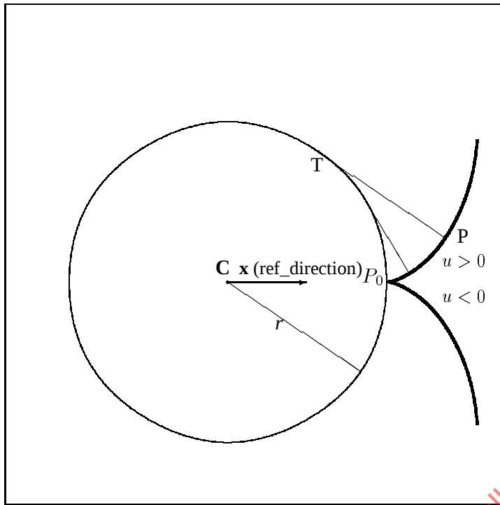
Figure 9 – Circular involute curve
