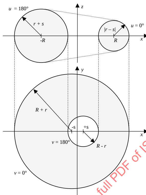
Figure 14 – Cross-sections of a Dupin cyclide with C = 0
