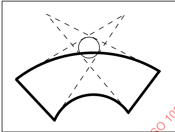
Figure 25 – Cross section of cyclide segment_solid
