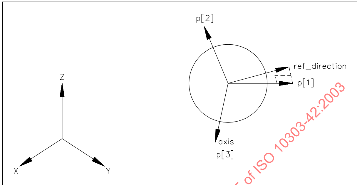
Figure 4 – Circle
