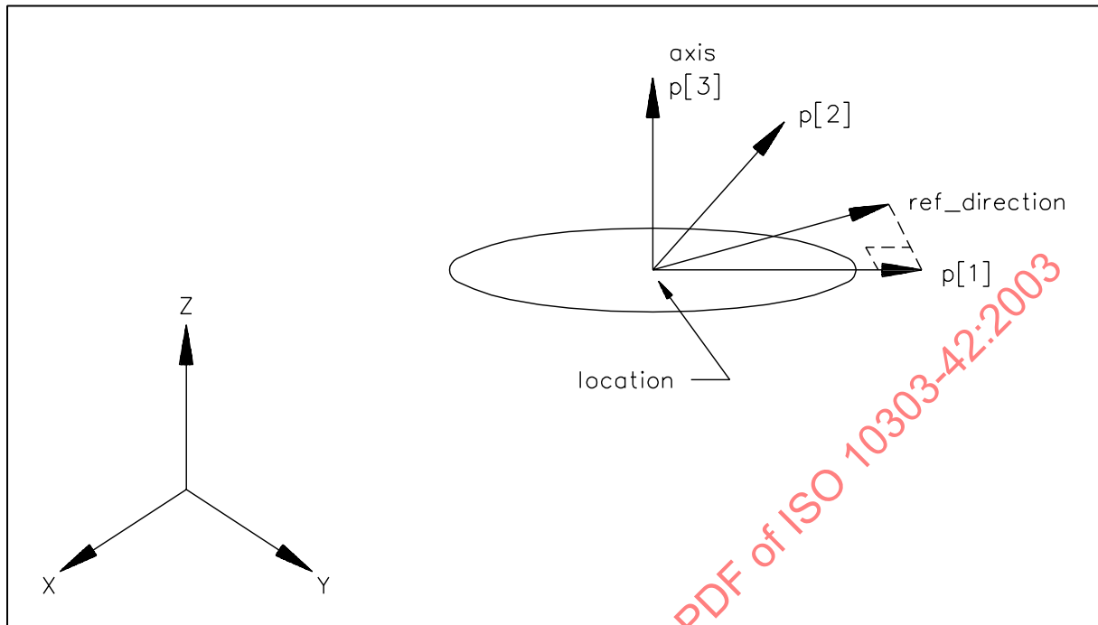
Figure 5 – Ellipse
