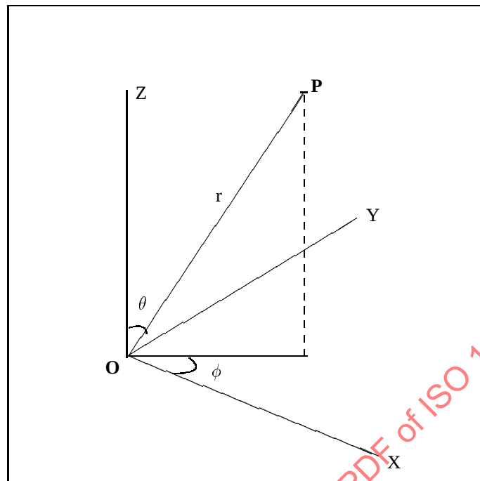
Figure 1 – Spherical_point attributes
