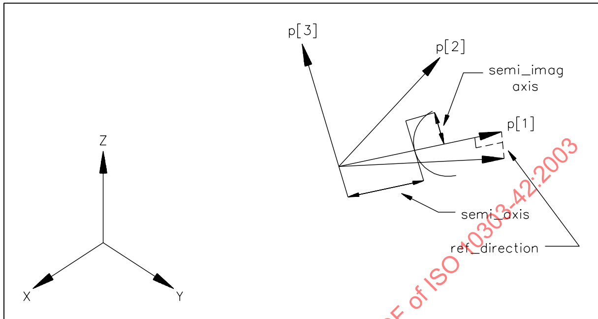
Figure 6 – Hyperbola
