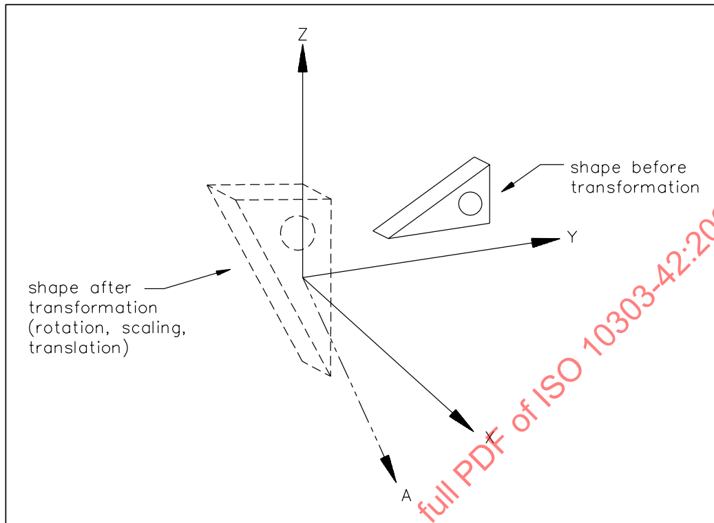
Figure 3 – (c) Cartesian_transformation_operator_3d
