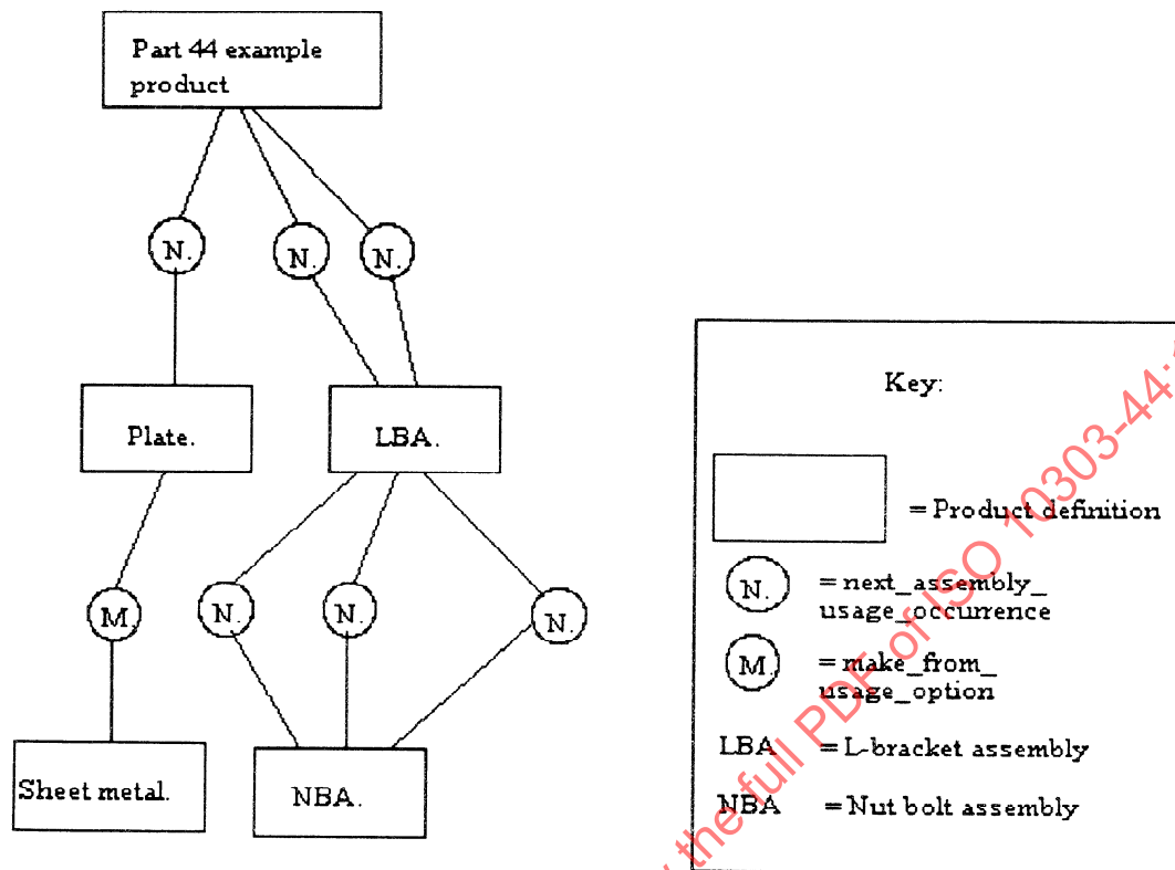
Figure E.5 - BOM data structure examples using Part 44 entities
