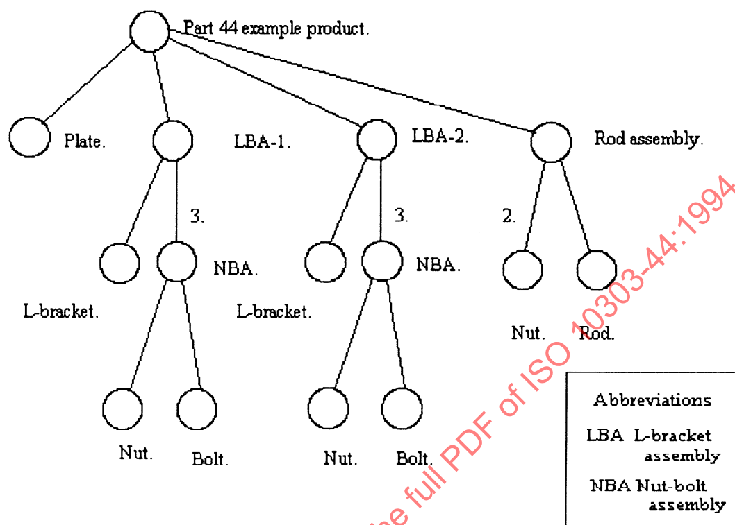
Figure E.2 - Part 44 example product: graphical product structure
