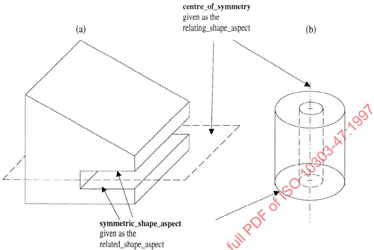
Figure 3 - Symmetry_shape_aspect and centre_of_symmetry
