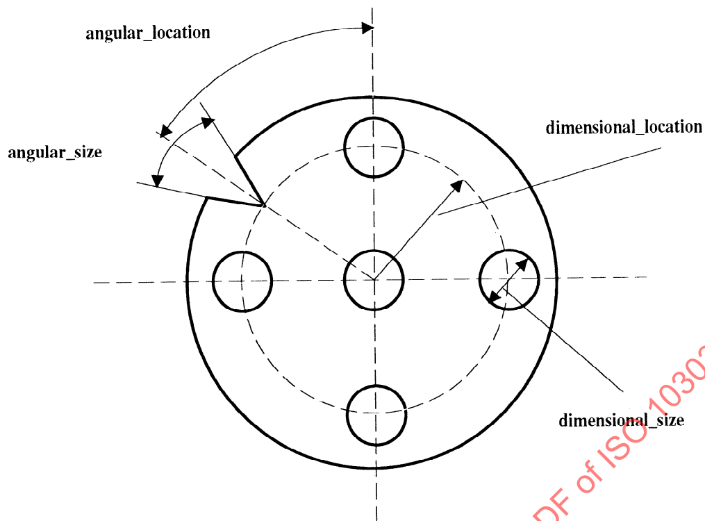
Figure 11 - Dimensional_location and dimensional_size
