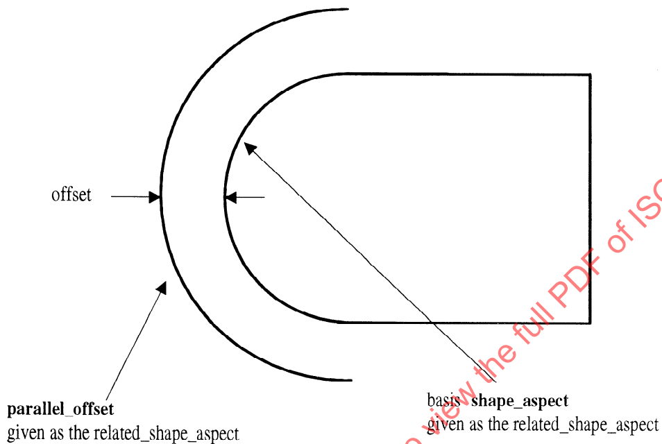
Figure 6 - Parallel_offset
