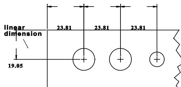
Figure 7 - Chain dimension pair
