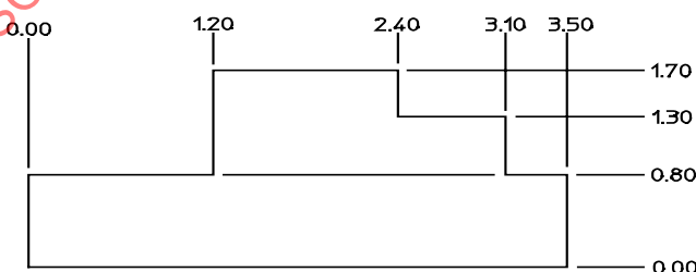
Figure 9 - Ordinate dimension
