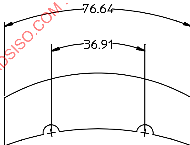
Figure 2 - Curve dimension
