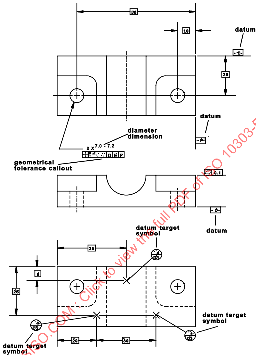
Figure 3 - Draughting callouts
