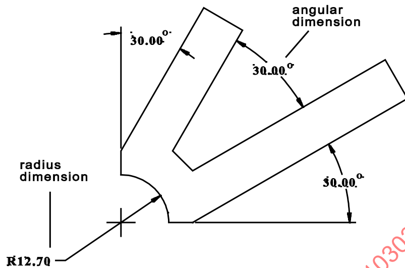
Figure 1 - Angular and radius dimensions
