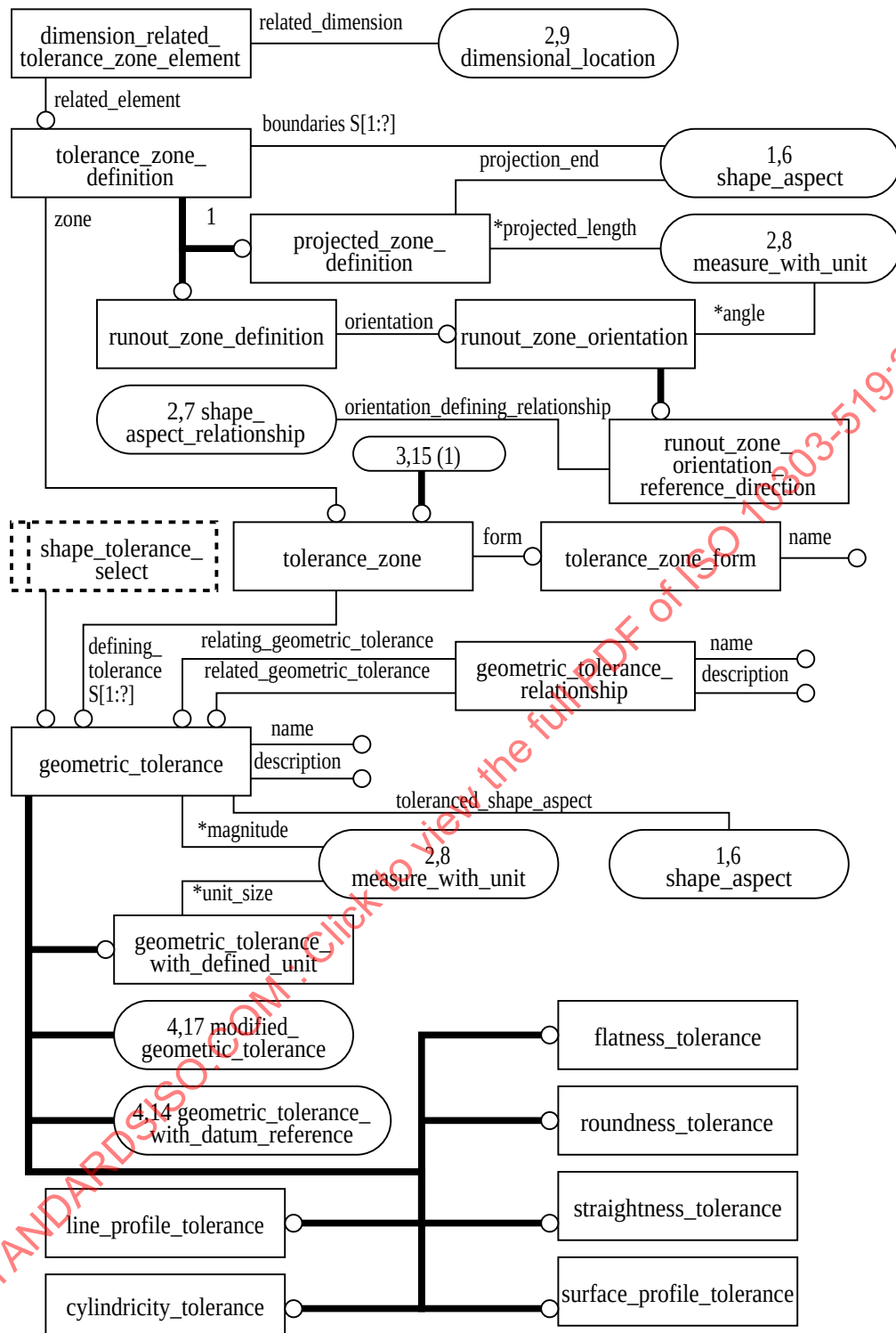
Figure C.3 – AIC expanded listing diagram in EXPRESS-G:
