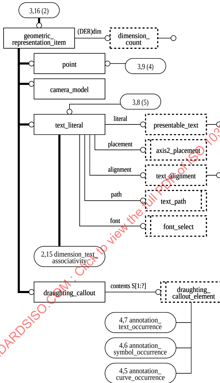
Figure C.3 – AIC expanded listing diagram in EXPRESS-G: 3 of 6
