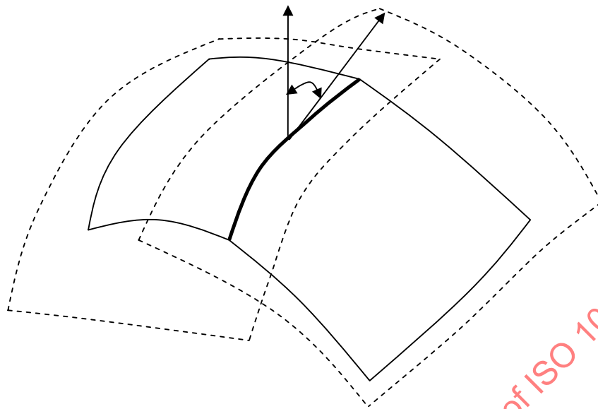
Figure 40 – Measurement of G1 discontinuity between faces
