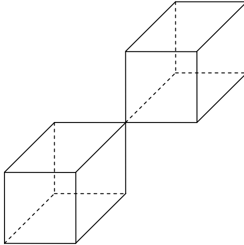
Figure 17 – Non-manifold vertex
