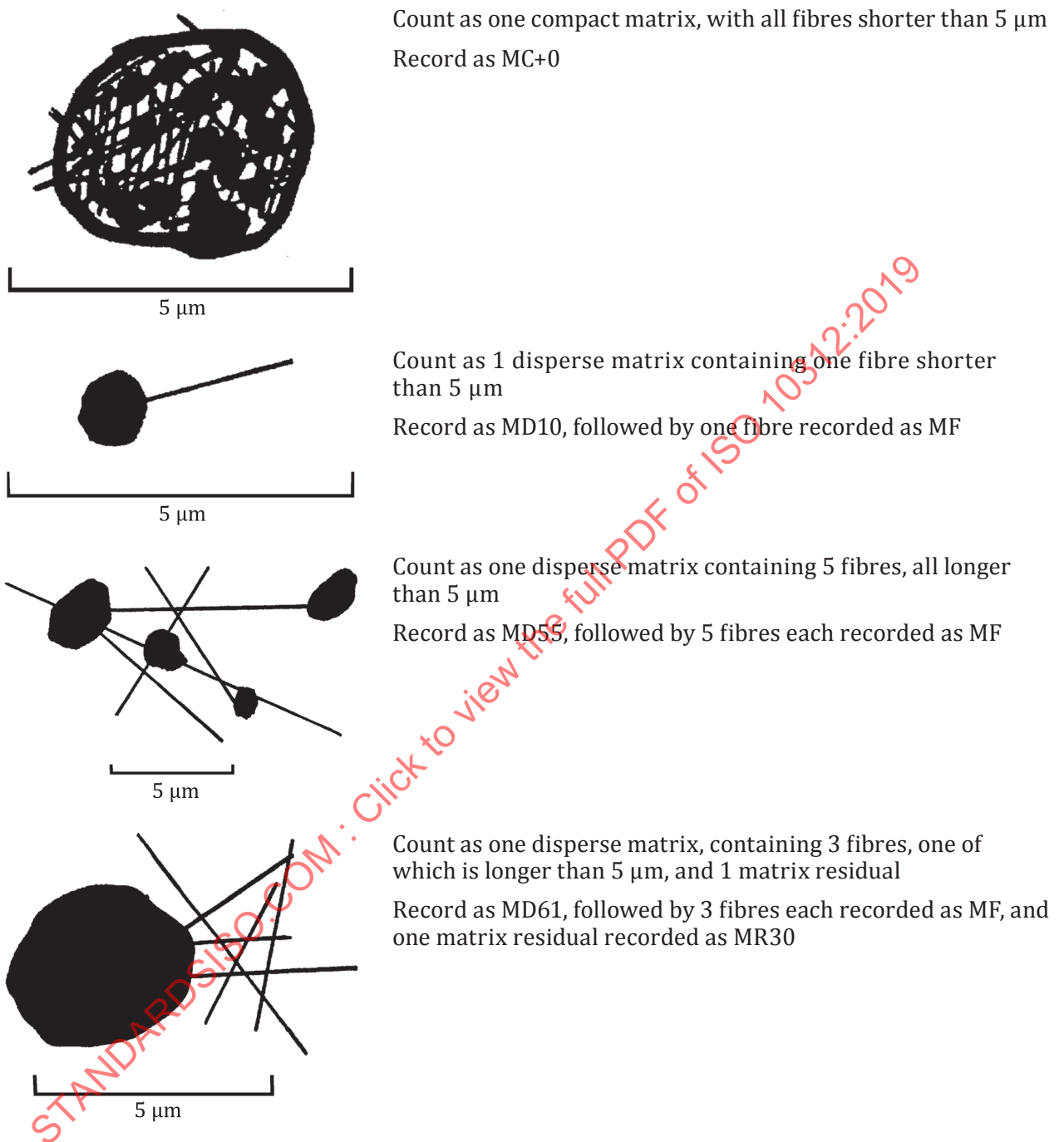
Figure C.3 — Examples of recording of complex asbestos matrices
