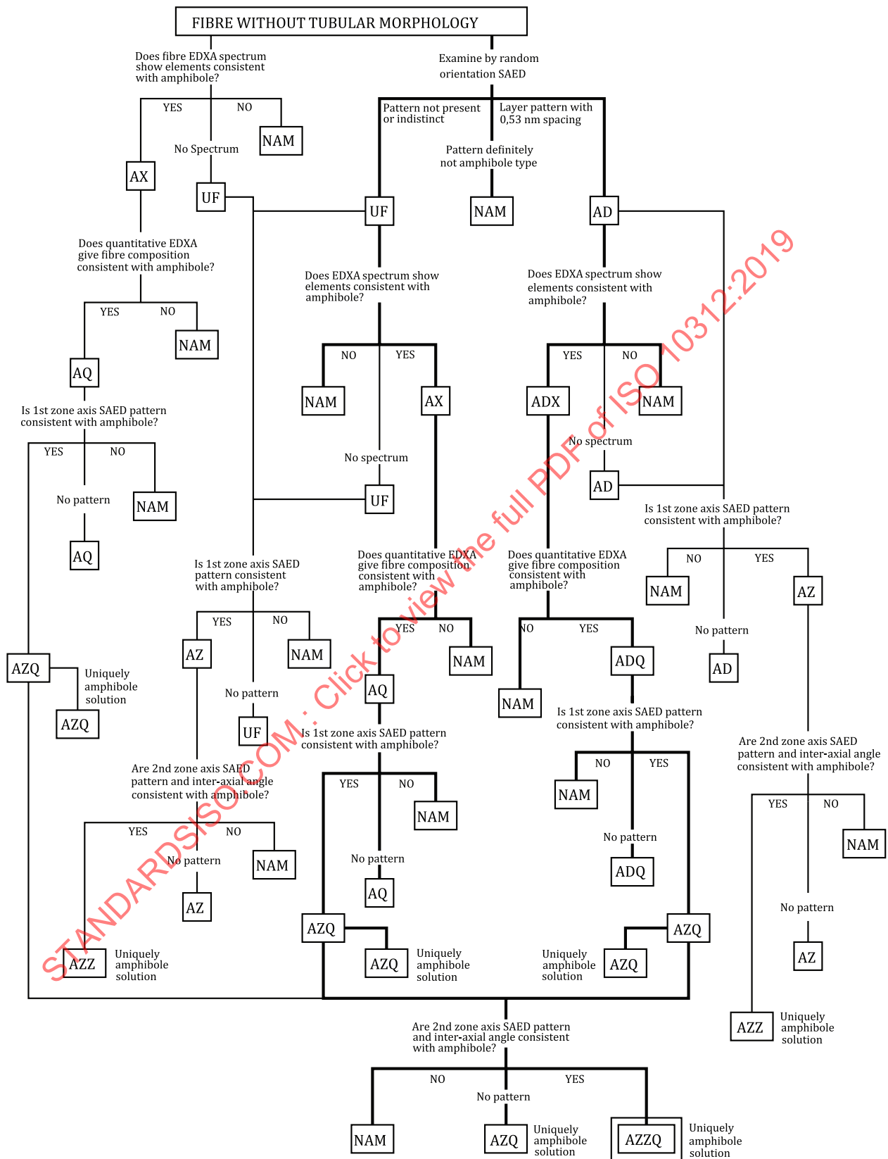
Figure D.4 — Classification chart for fibre without tubular morphology
