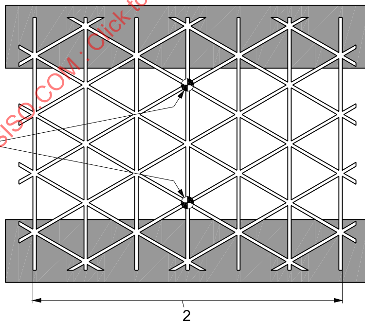
Figure 6 — Example of geogrid with three axes, specimen size, widths and gauge length MD
