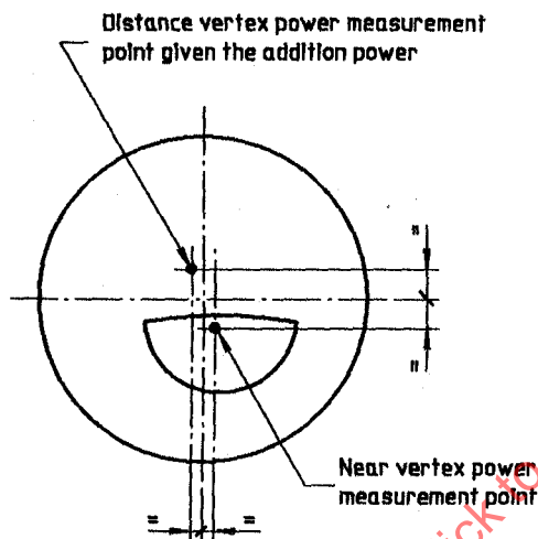
Figure 2 — Measurement of the distance vertex power
