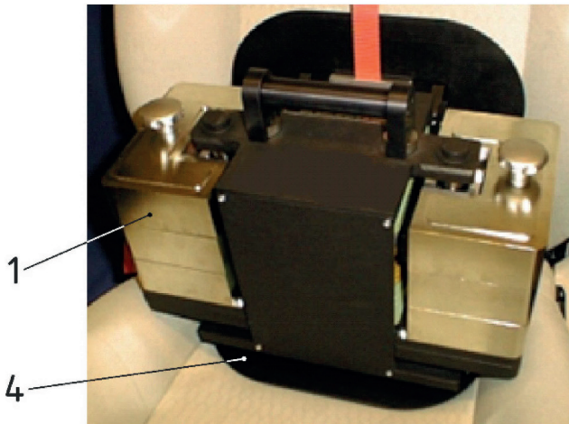
a) Example of passive dynamic dummy used for sea tests
