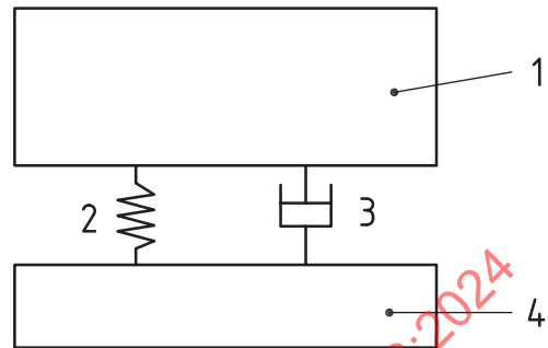
b) One-degree-of-freedom discrete-element model
