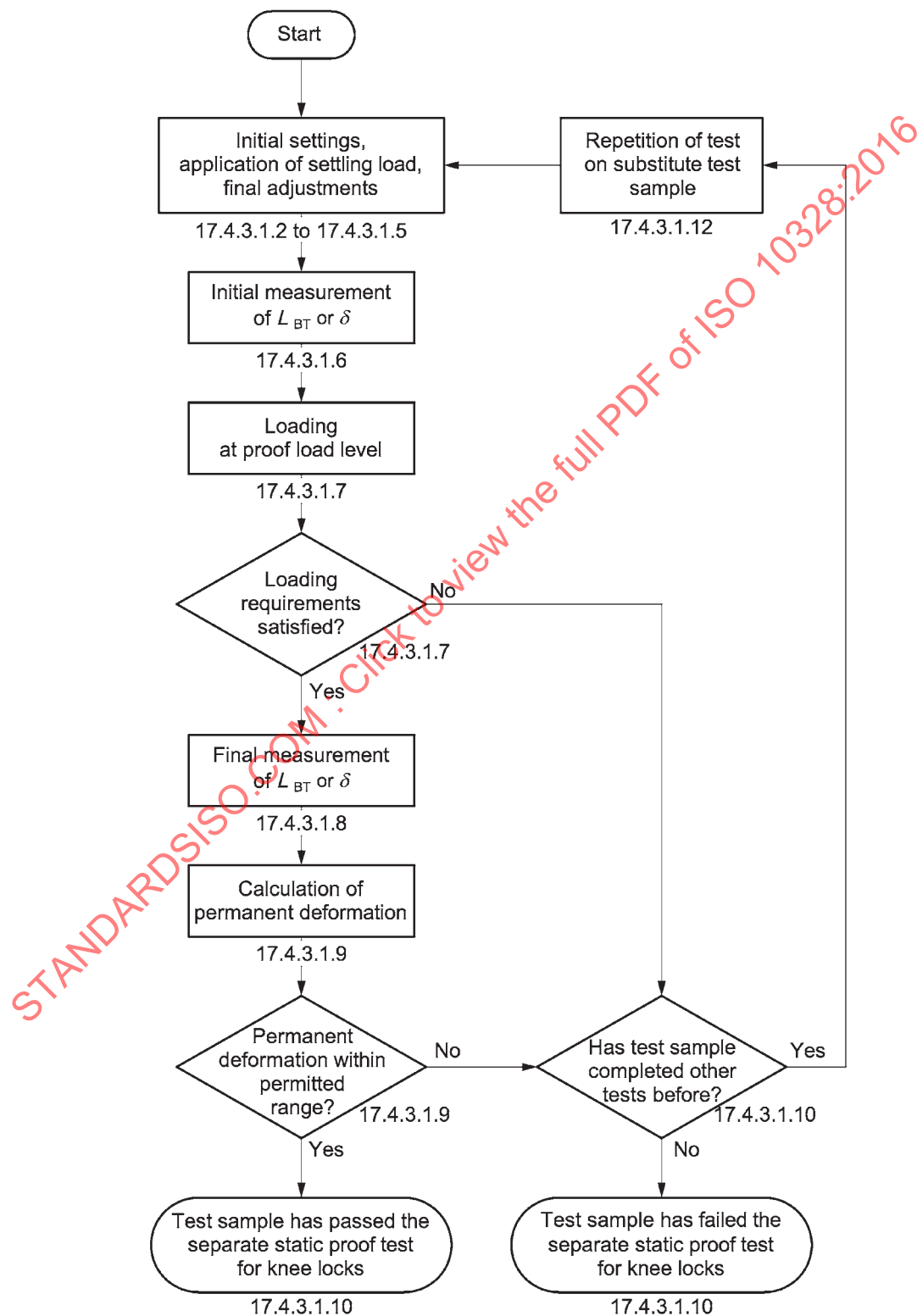
Figure 24 — Flowchart for the separate static proof test for knee locks, specified in 17.4.3.1
