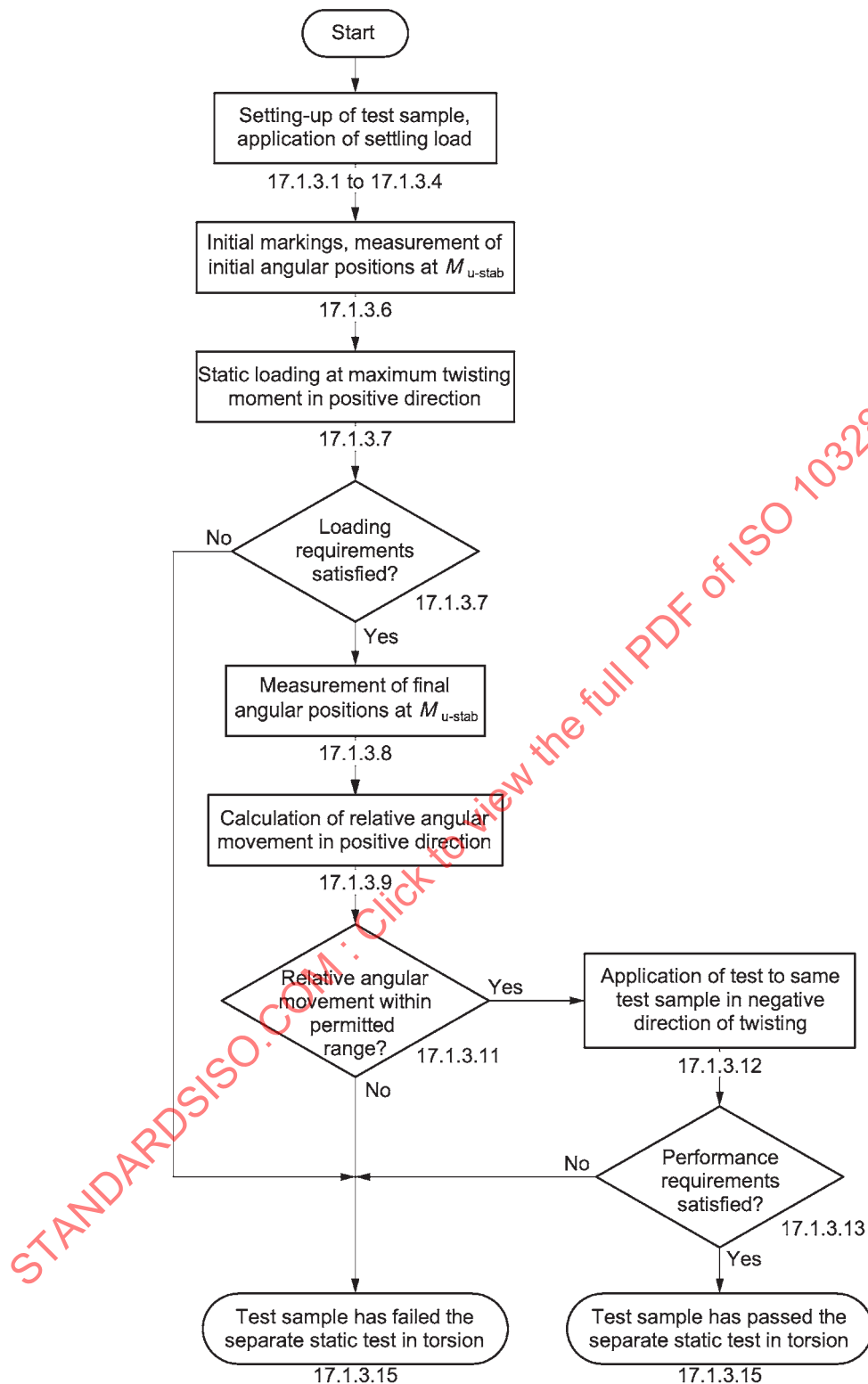
Figure 18 — Flowchart for the separate static test in torsion, specified in 17.1.3
