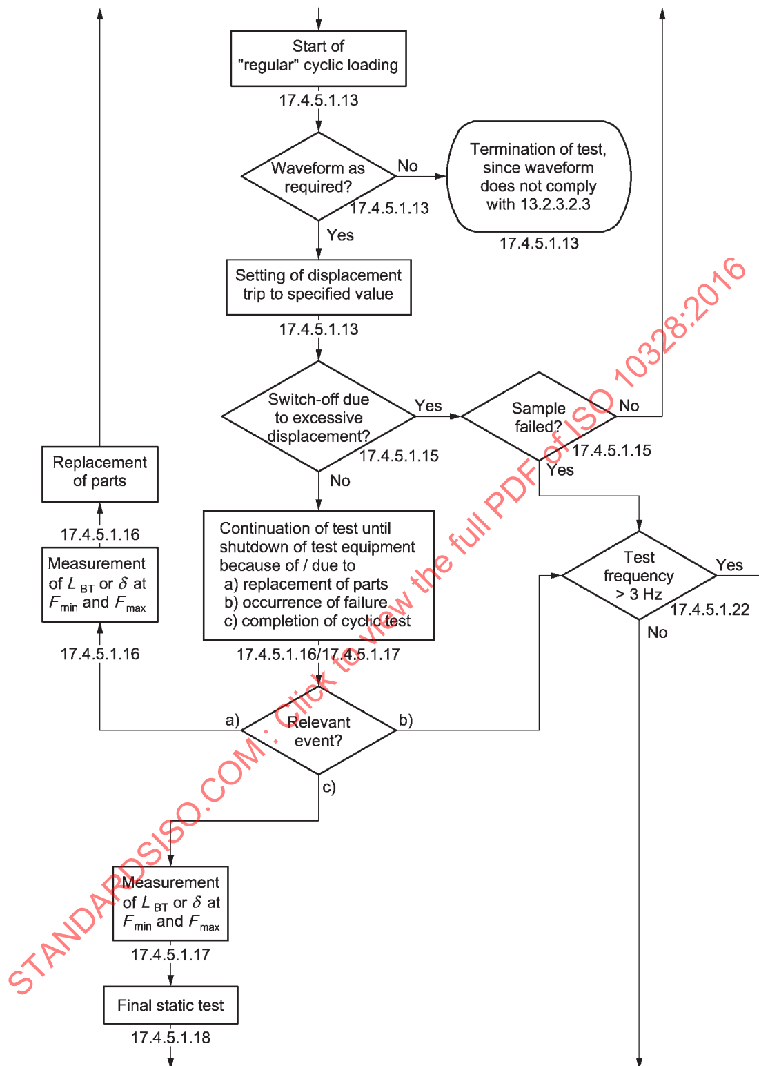
Figure 27 — Flowchart for the separate cyclic test for knee locks, specified in 17.4.5.1 Continued from Figure 26 and continued on Figure 28
