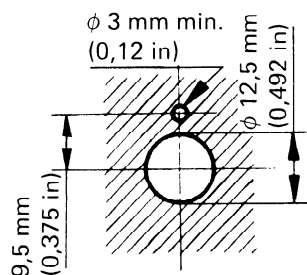
FIGURE 2 — Panel drilling
