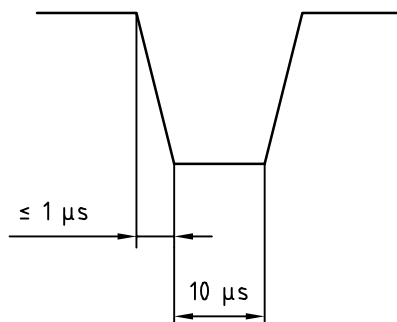
b) Input waveform at ignition circuit terminals
