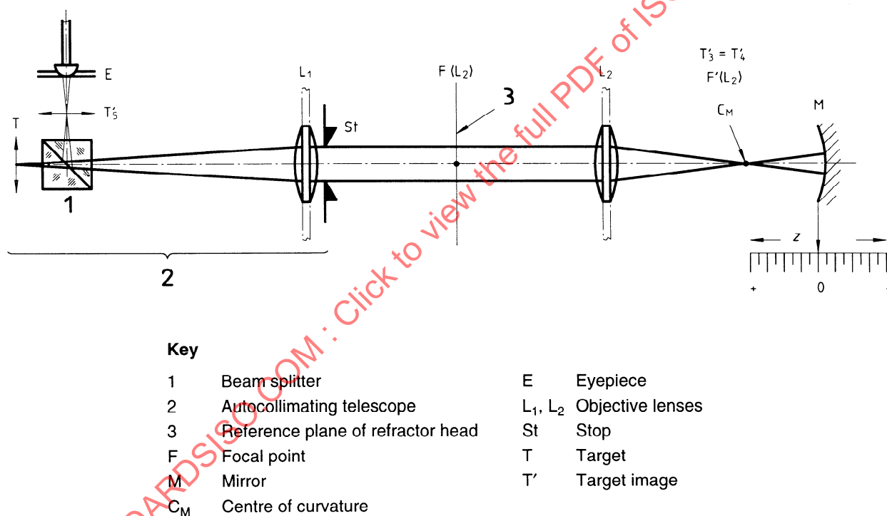
Figure A.1 — Setup for a refractor head test device
