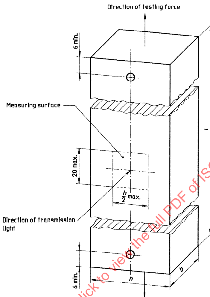
Figure 1 — Test specimen with holes
