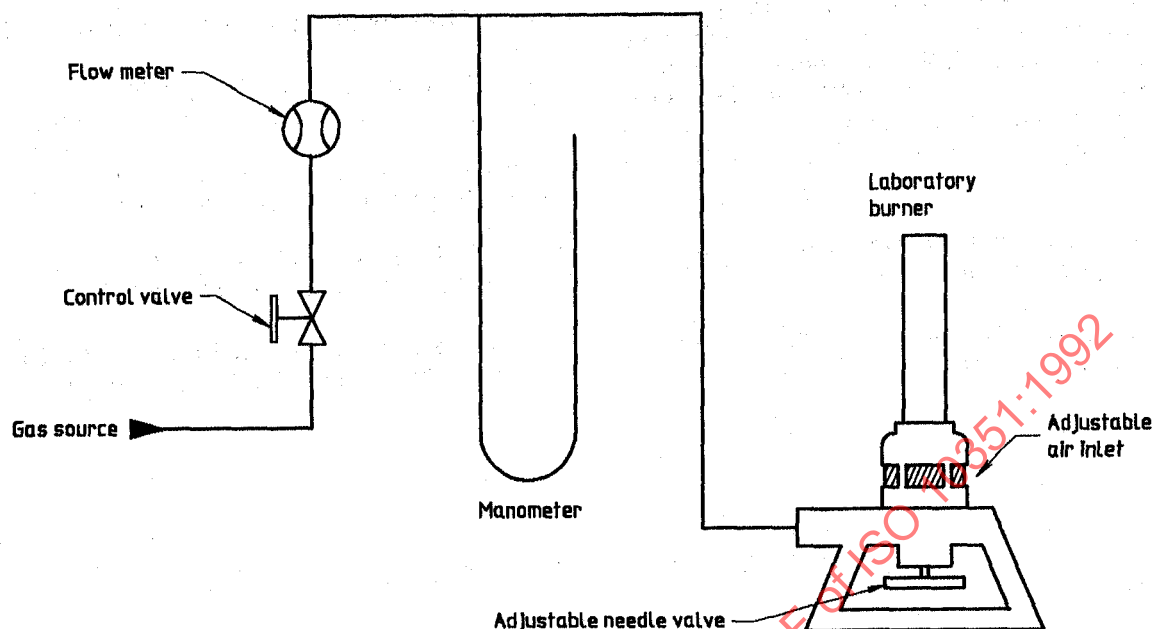
Figure A.3 — Burner supply arrangement
