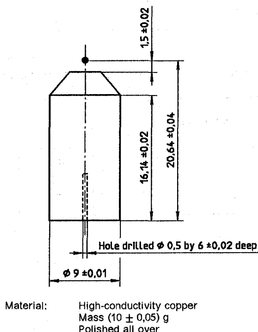
Figure A.1 — Thermal sensor
