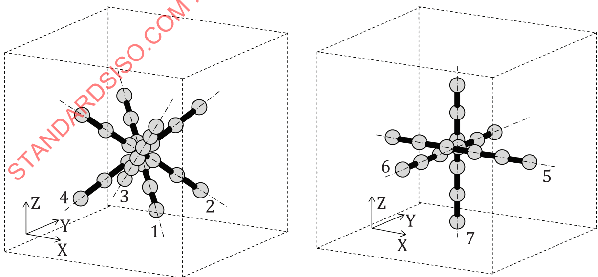
Figure 3 — Example of positions of material standards in the assessment: required four diagonal positions and default three positions along the axes of the coordinate system
