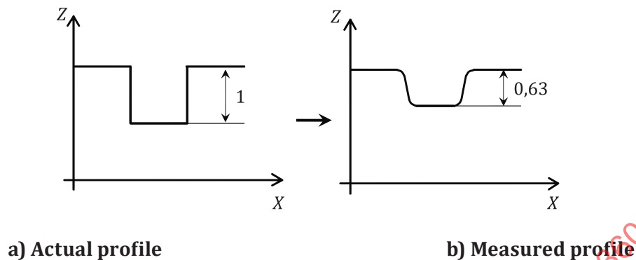
Figure F.1 — Verification of structural resolution using a structure standard with a gap or pit
