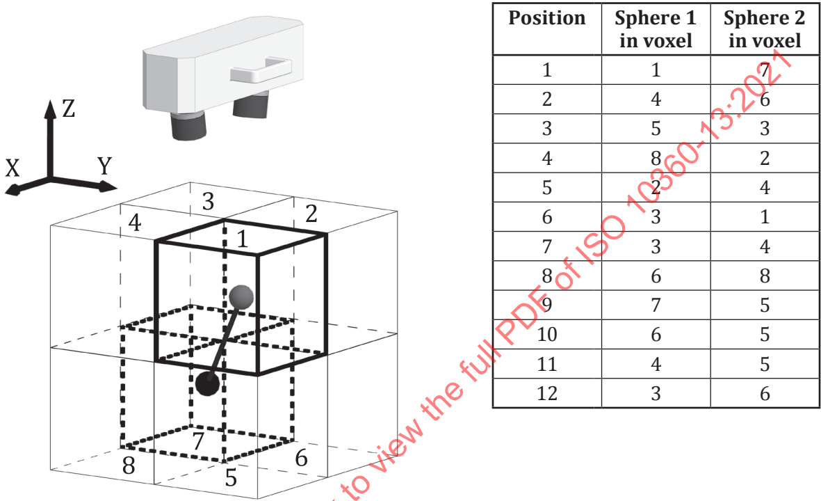
a) Positions of the calibrated test length in the sensor measurement volume, overview
