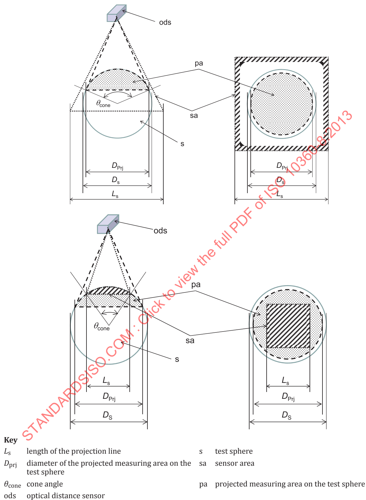
Figure 6 — Measuring area on the test sphere and cone angle to be reported
