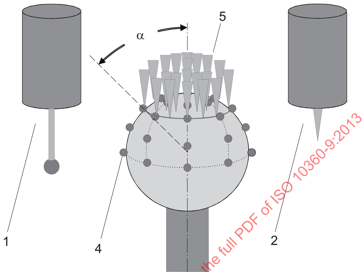
a) Contacting probe and optical distance probe
