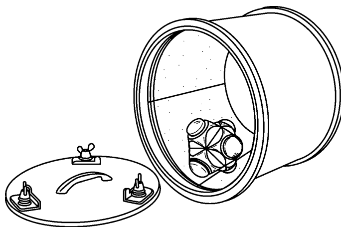
Figure 3 — Hexapod tumbler tester
