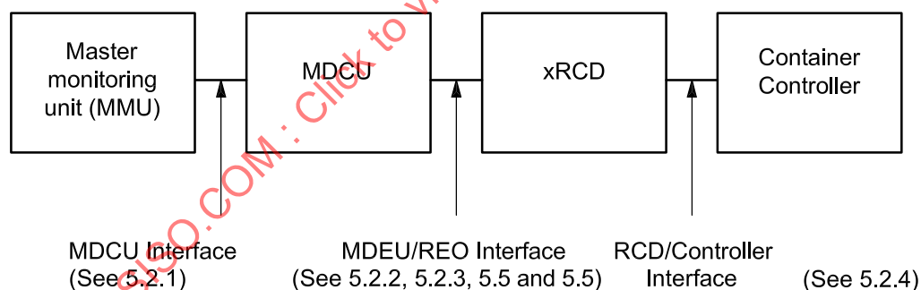
Figure 2 — Remote condition monitoring — Communications interfaces
