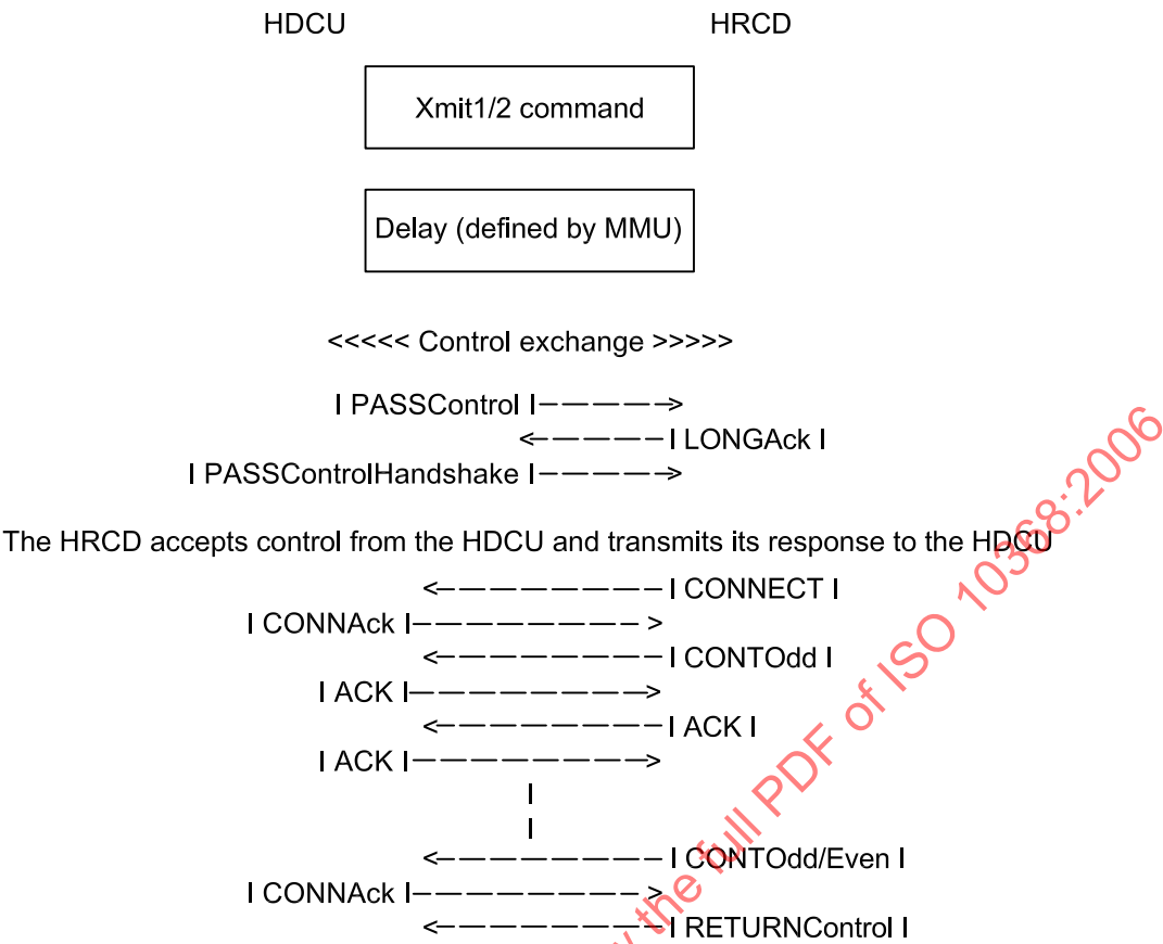
Figure 19 — RCD/device interactive1/2 session transfer diagram
