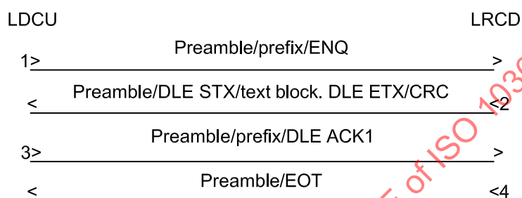
Figure 10 — Poll session transfer diagram
