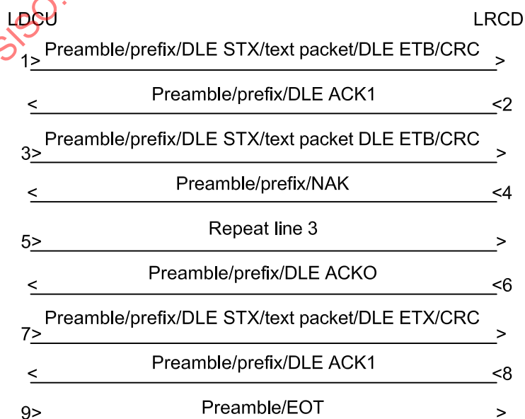
Figure 11 — Xmit1 session transfer diagram
