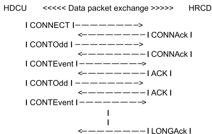
Figure 18 — RCD/device xmit1/2 session transfer diagram
