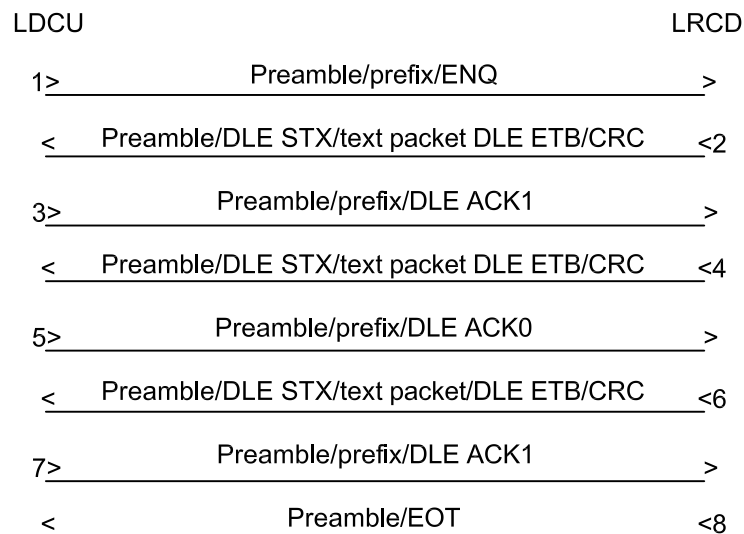
Figure 15 — Interactive poll session transfer diagram
