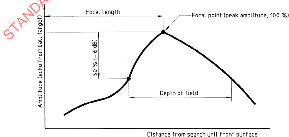
Figure 10 — Axial beam profile of a focused-beam immersion search unit
