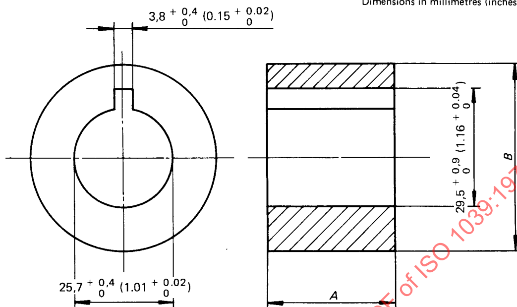
FIGURE 1 – Dimensions common to all simple cores
