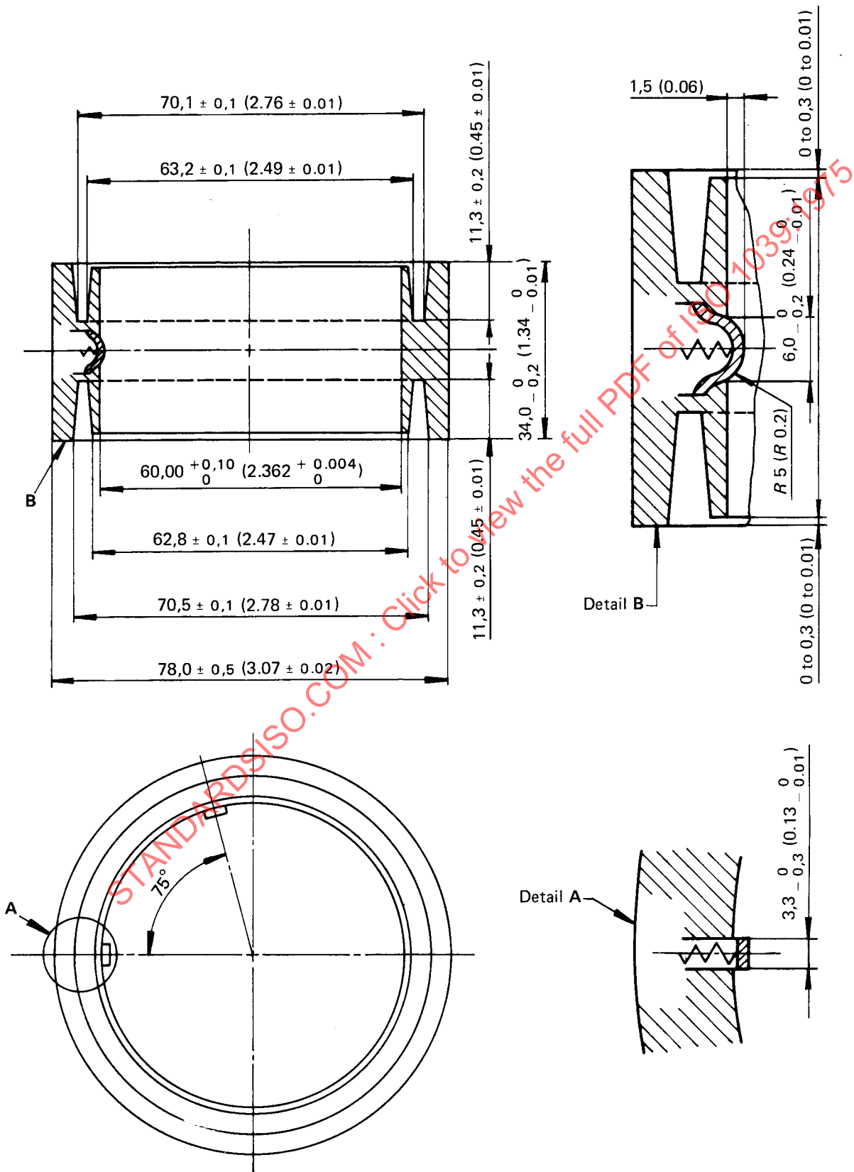
FIGURE 3 – Dimensions for core with light lock groove
