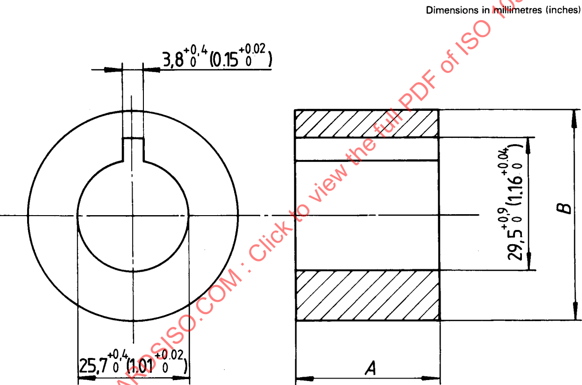
Figure 1 — Dimensions common to all simple cores
