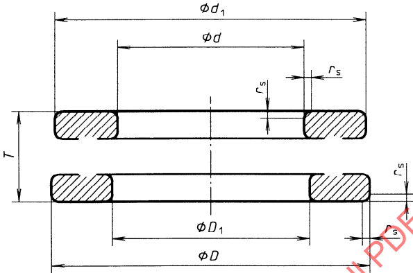
Figure 1 — Single-direction thrust bearing
