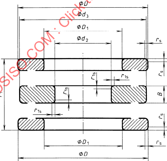
Figure 2 — Double-direction thrust bearing
