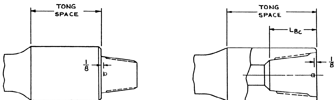
FIG. 10.5 TONG SPACE AND BENCH MARK POSITION
