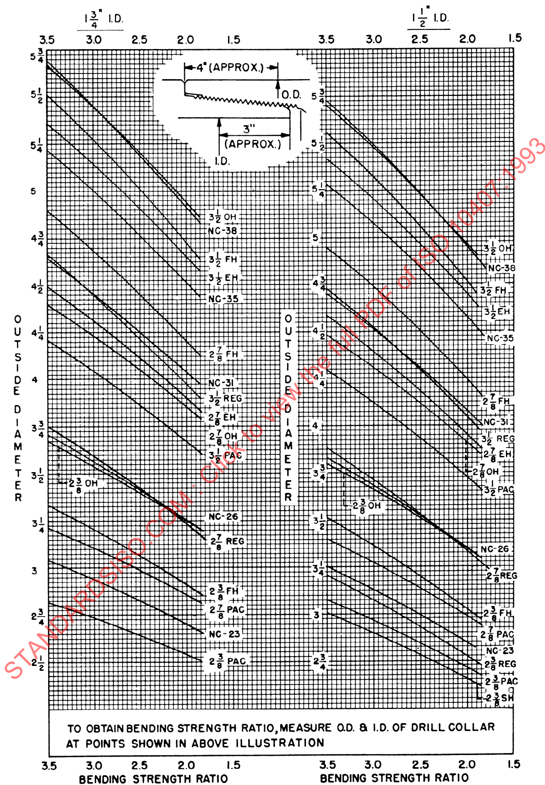
FIG. 3.1 DRILL COLLAR BENDING STRENGTH RATIOS, 1 1/2 AND 1 3/4 INCH ID
