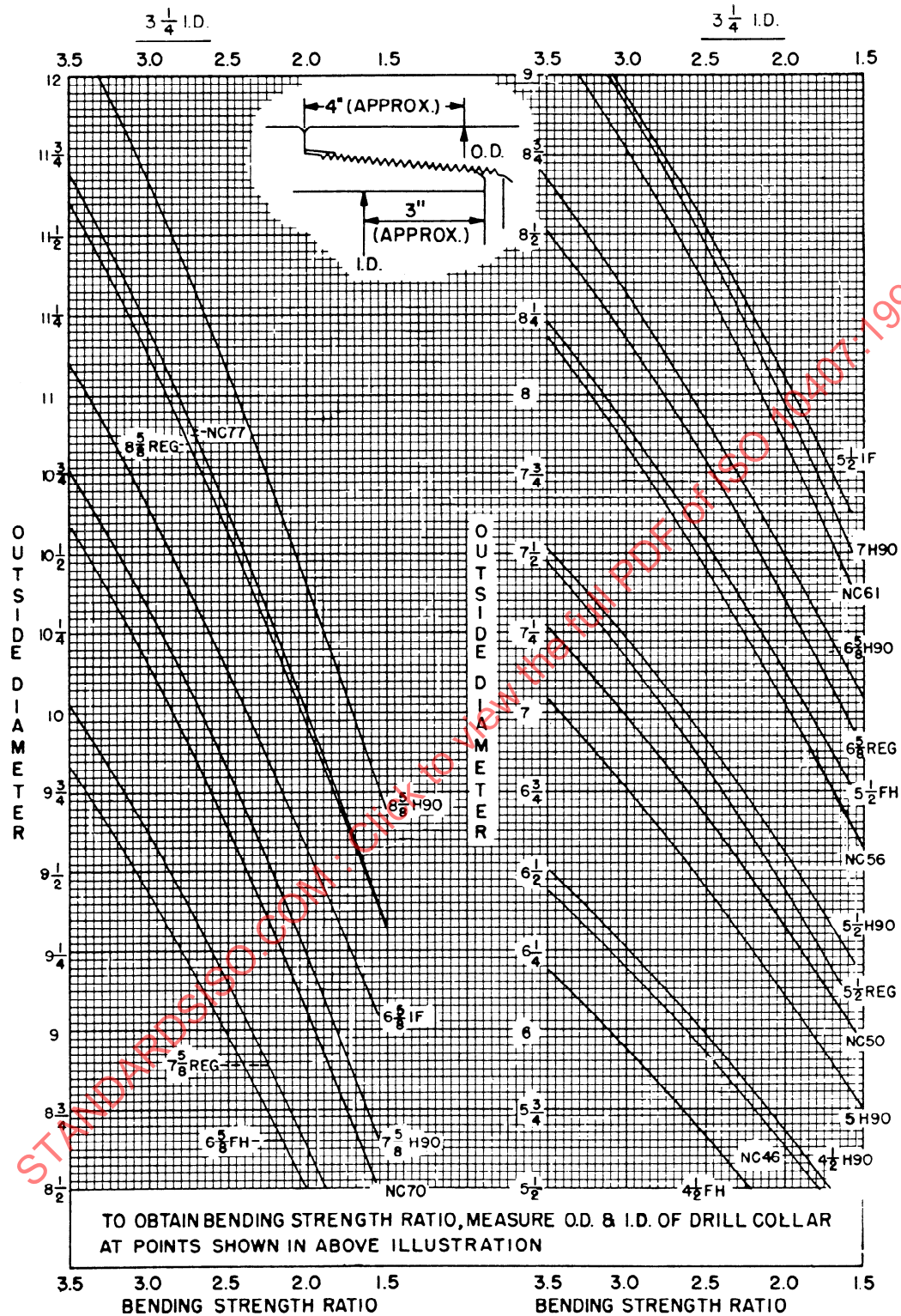
FIG. 3.6 DRILL COLLAR BENDING STRENGTH RATIOS, 3 1/4 INCH ID
