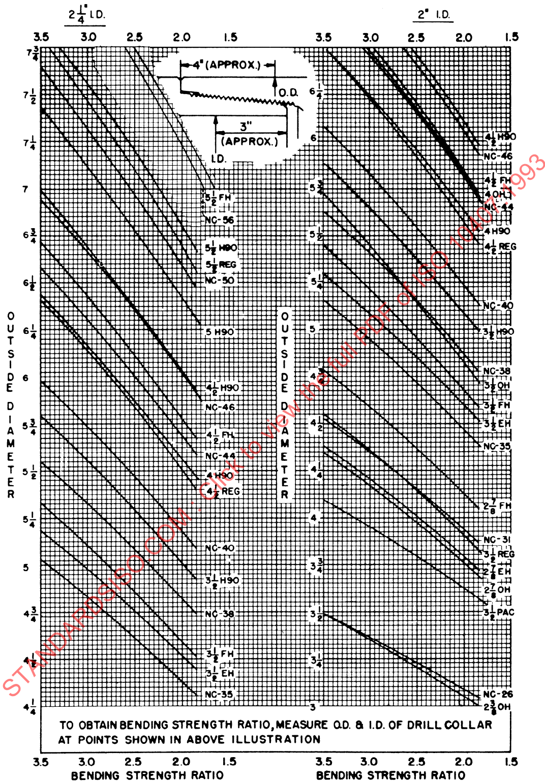
FIG. 3.2 DRILL COLLAR BENDING STRENGTH RATIOS, 2 AND 2 1/4 INCH ID
