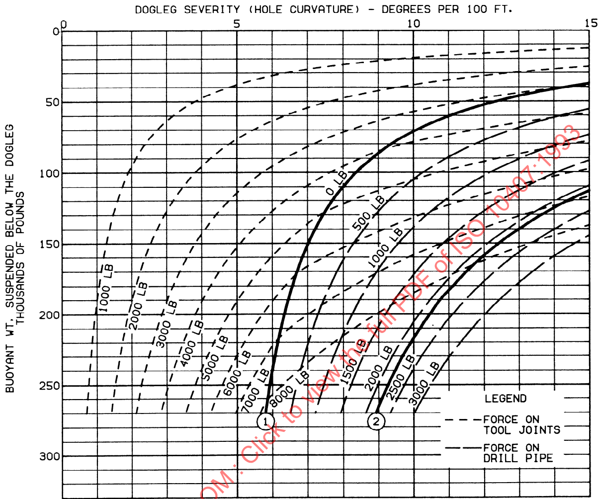
FIG. 6.7 LATERAL FORCES ON TOOL JOINTS AND RANGE 2 DRILL PIPE 4½", 16.6 LB PER FOOT, RANGE 2 DRILL PIPE, 6¼" TOOL JOINTS
