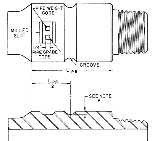
STANDARD WEIGHT HIGH STRENGTH DRILL PIPE
