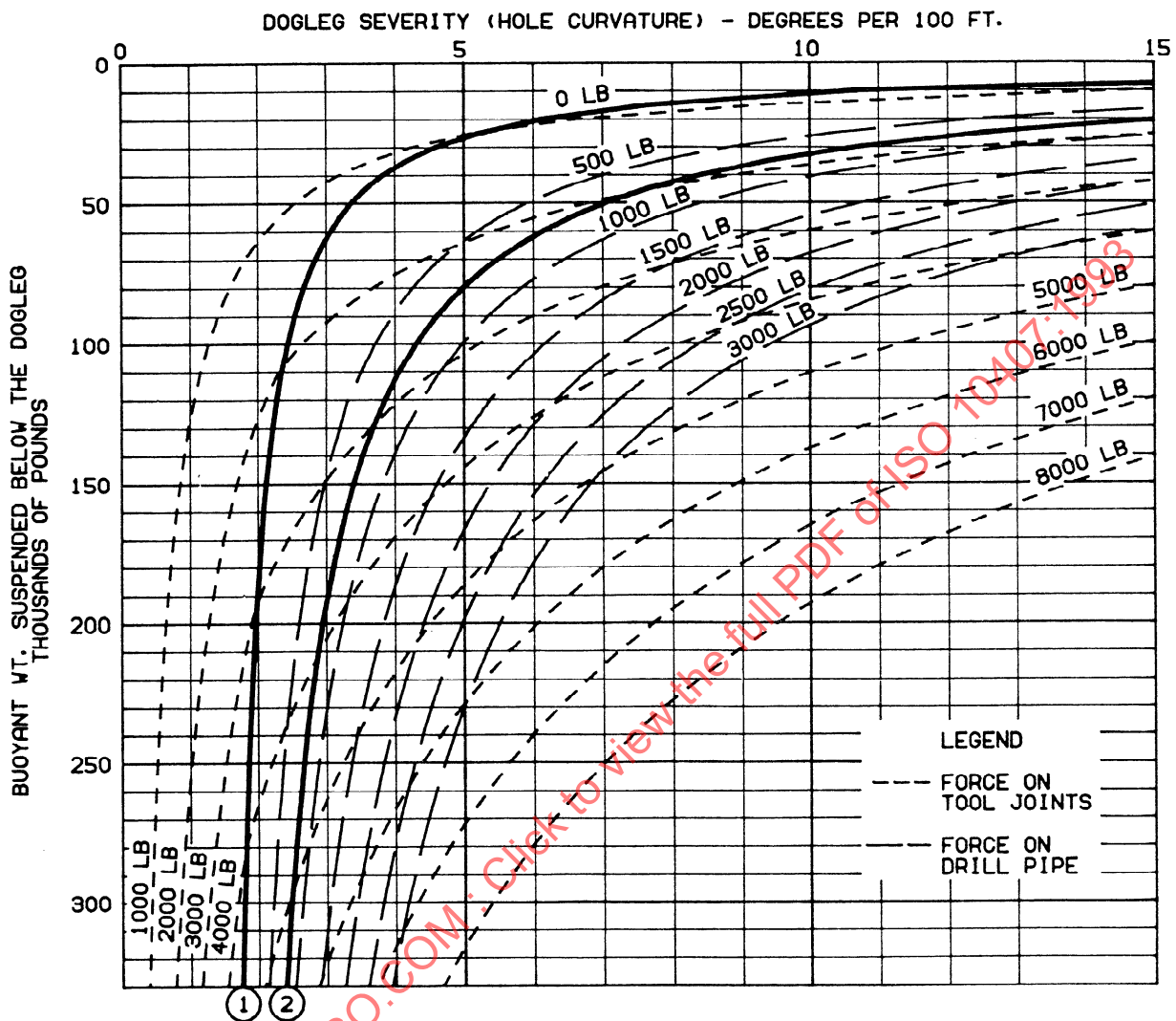
FIG. 6.9 LATERAL FORCES ON TOOL JOINTS AND RANGE 3 DRILL PIPE 5" 19.5 LB PER FOOT, RANGE 3 DRILL PIPE, 6 3/8" TOOL JOINTS
