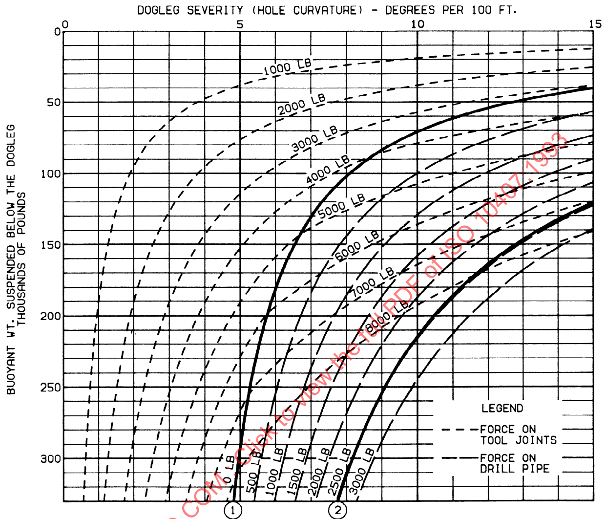
FIG. 6.8 LATERAL FORCES ON TOOL JOINTS AND RANGE 2 DRILL PIPE 5", 19.5 LB PER FOOT, RANGE 2 DRILL PIPE, 6 3/8" TOOL JOINTS
