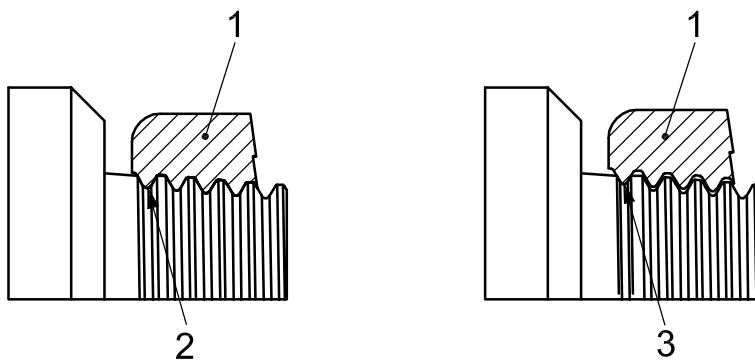
Figure 14 — Location of last full-depth thread
