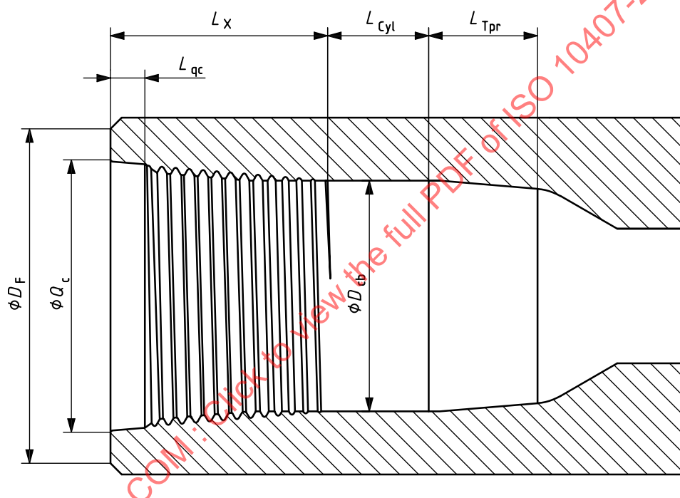
Figure 13 — Boreback box
