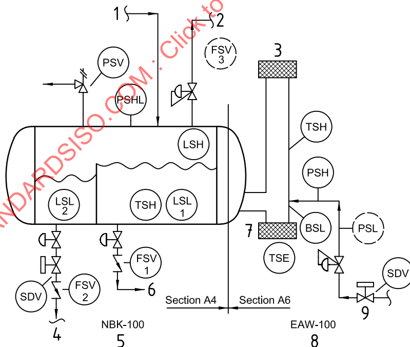
Figure C.4 — Simplified diagram showing required safety devices
