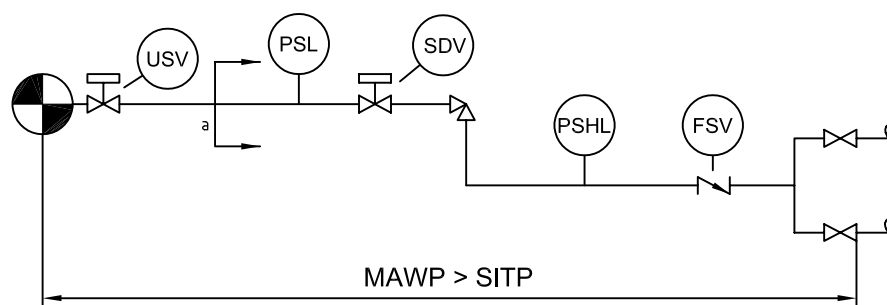
Figure B.2 — Recommended safety devices — Underwater wellhead flowlines
