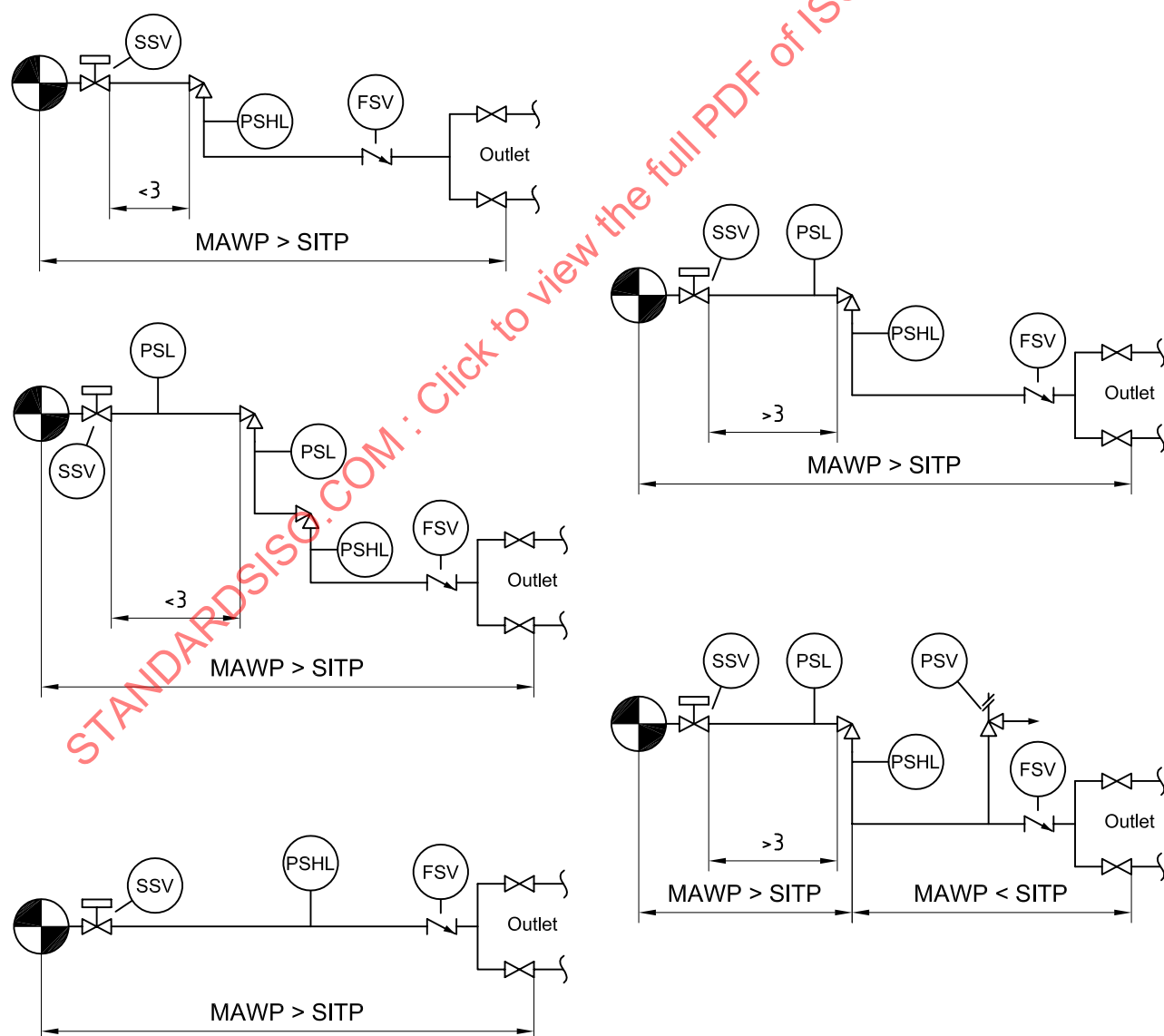
Figure B.1 — Recommended safety devices — Typical wellhead flowlines
