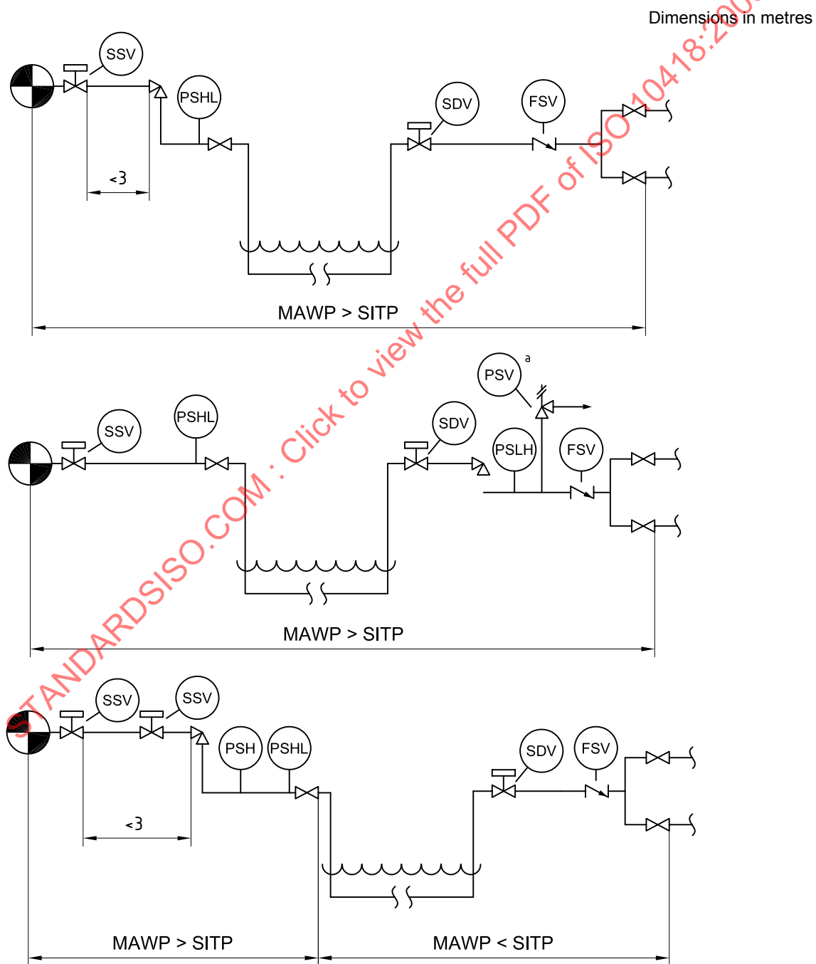
Figure B.3 — Recommended safety devices — Satellite well
