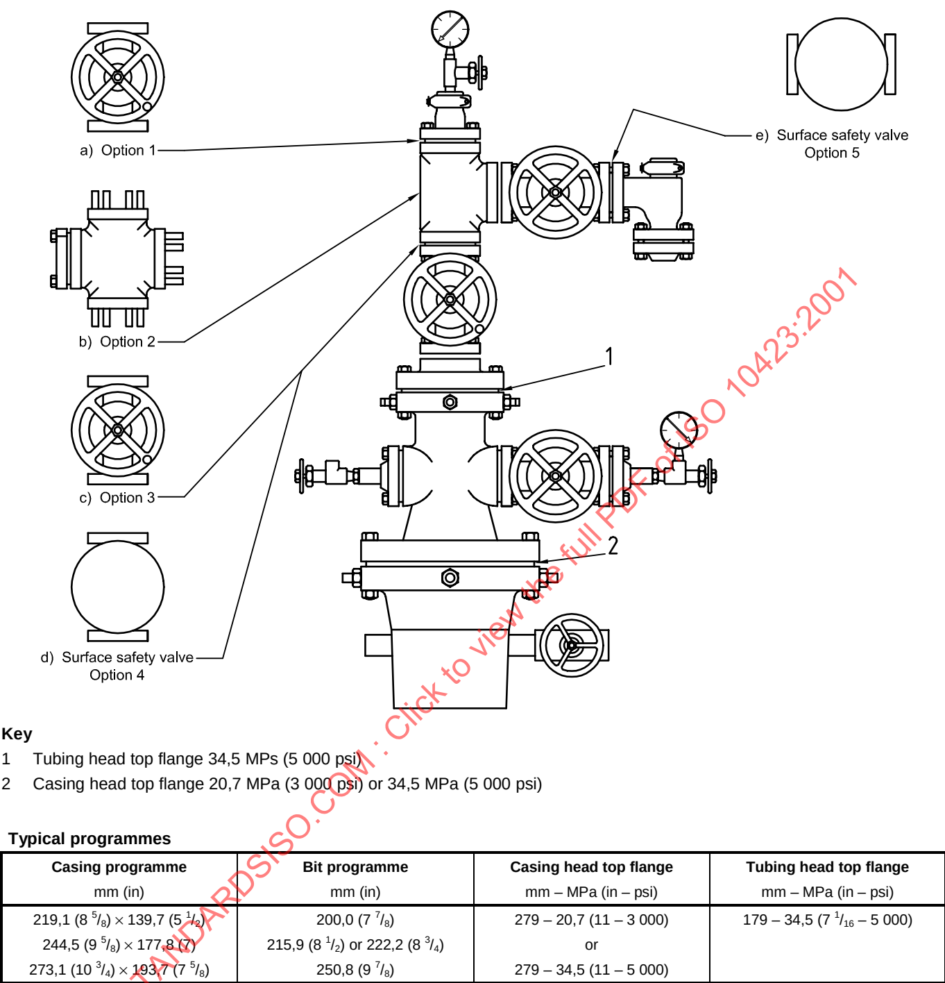
Figure A.1 — Typical wellhead and tree configuration 34,5 MPa (5 000 psi) rated working pressure
