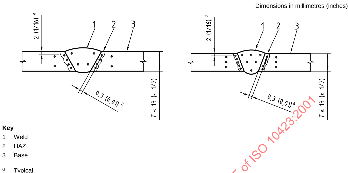
Figure 5 — Welding procedure qualification — Vickers hardness test locations (PSL 3)
