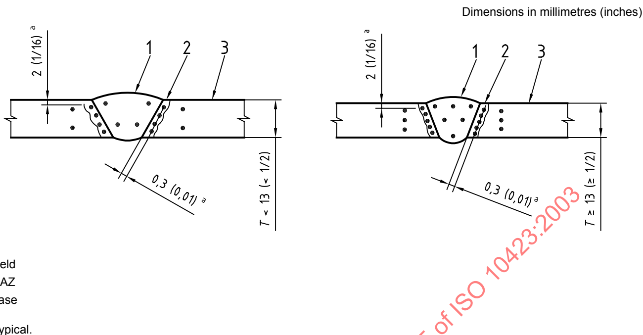
Figure 5 — Welding procedure qualification — Vickers hardness test locations (PSL 3)
