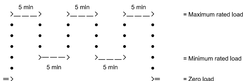
Figure F.2 — Load cycle testing for hangers
