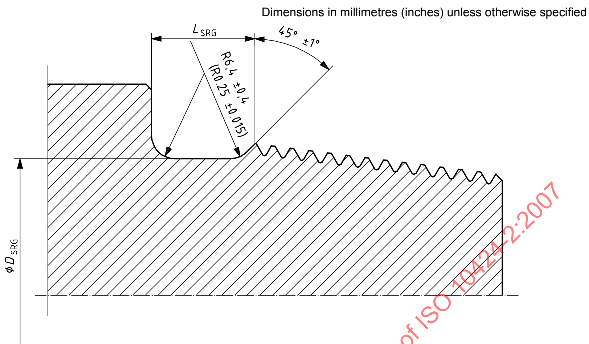
Figure 9 — Pin stress-relief groove
