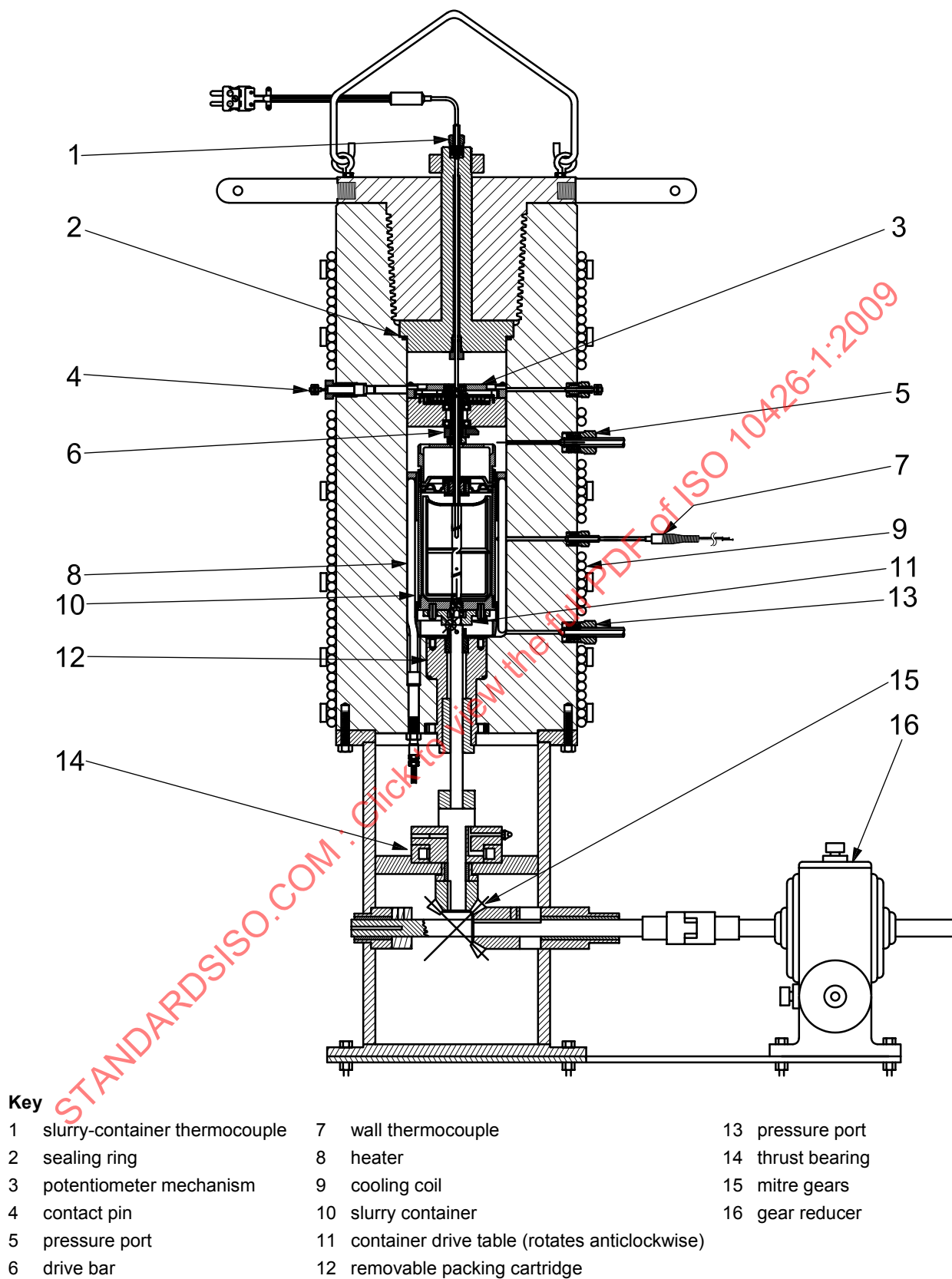
Figure 8 — Typical gear drive consistometer for pressurized specification thickening-time test
