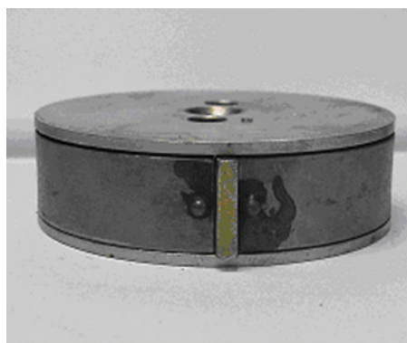
Figure 6 — Mould with a spacer block (side view)
