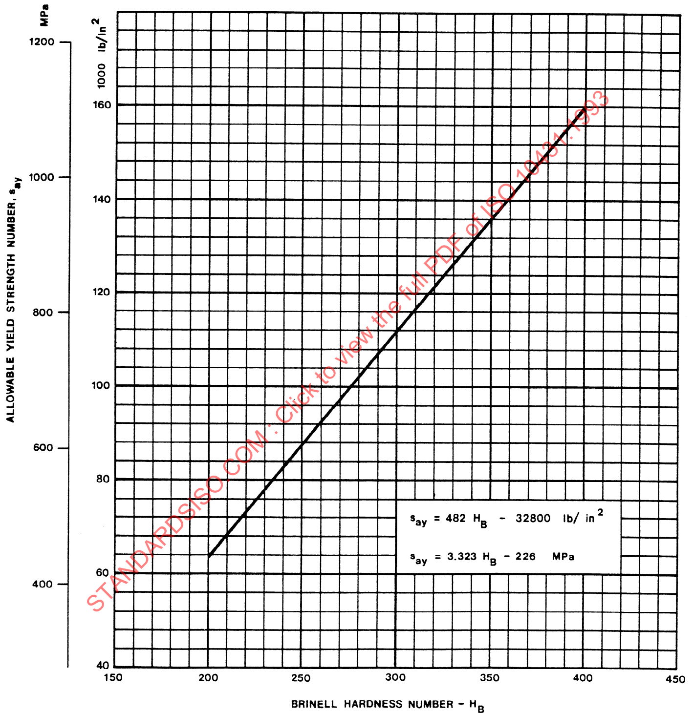
FIG. 3.9 ALLOWABLE YIELD STRENGTH NUMBER — s_{ay} STEEL AND NODULAR IRON FROM AGMA 422.03
