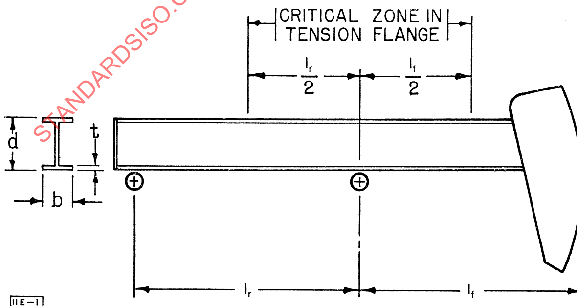
FIG. 2.1 WALKING-BEAM ELEMENTS
