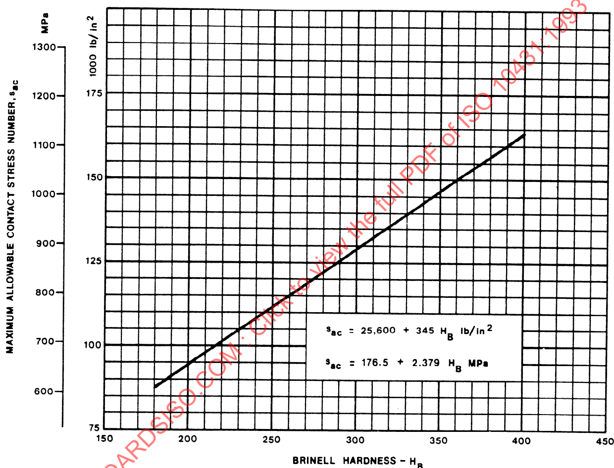
FIG. 3.1 ALLOWABLE CONTACT FATIGUE STRESS FOR THROUGH HARDENED AND TEMPERED STEEL GEARS — s_{ac} FROM AGMA 422.03
