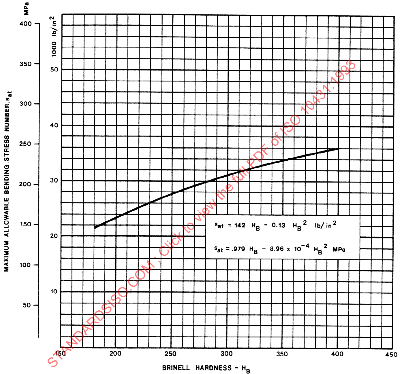
FIG. 3.3 ALLOWABLE BENDING FATIGUE STRESS FOR THROUGH HARDENED AND TEMPERED STEEL GEARS — s_{at} FROM AGMA 422.03
