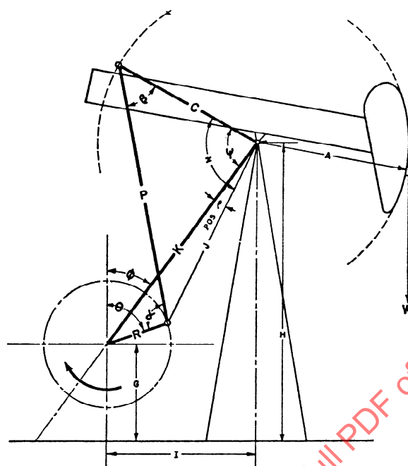
UPSTROKE
