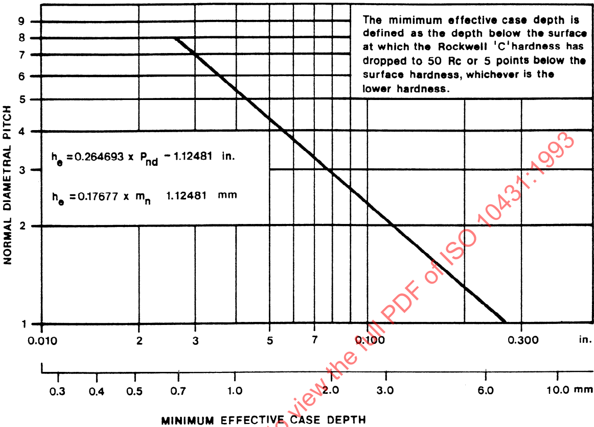
FIG. 3.7 MINIMUM EFFECTIVE CASE DEPTH FOR FLAME OR INDUCTION HARDENED GEARS, h_e FROM AGMA 422.03
