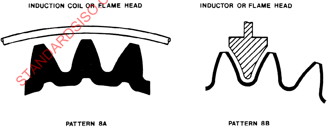
FIG. 3.8 ACCEPTABLE FLAME AND INDUCTION HARDENING PATTERNS FROM AGMA 422.03
