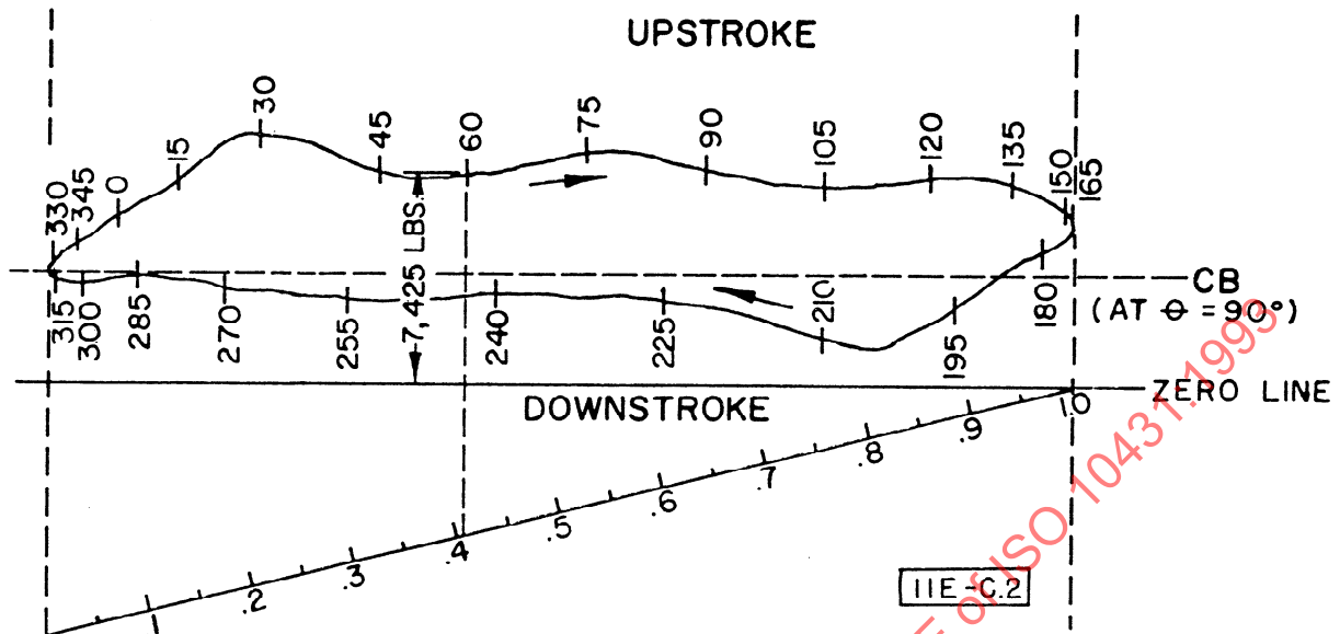
FIG. C2 DIVISION OF DYNAMOMETER CARD BY CRANK ANGLE USING API POLISHED-ROD POSITION DATA
