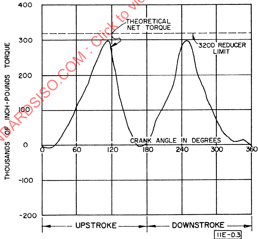
FIG. D3 TORQUE CURVES USING API TORQUE FACTORS
