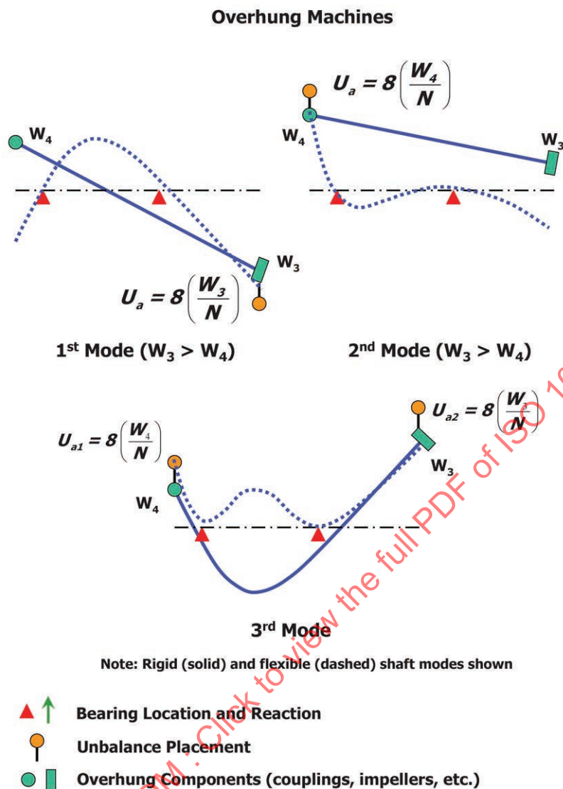
Figure 1 — Typical mode shapes and corresponding unbalance
