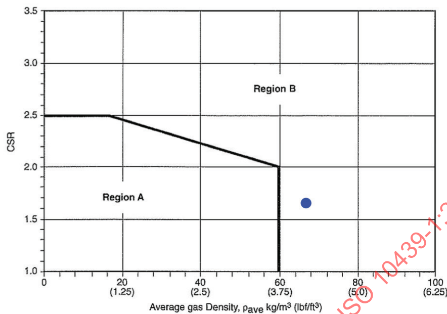
Figure C.3 — Stability experience plot
