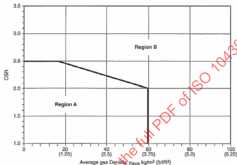
Figure 4 — Stability experience plot
