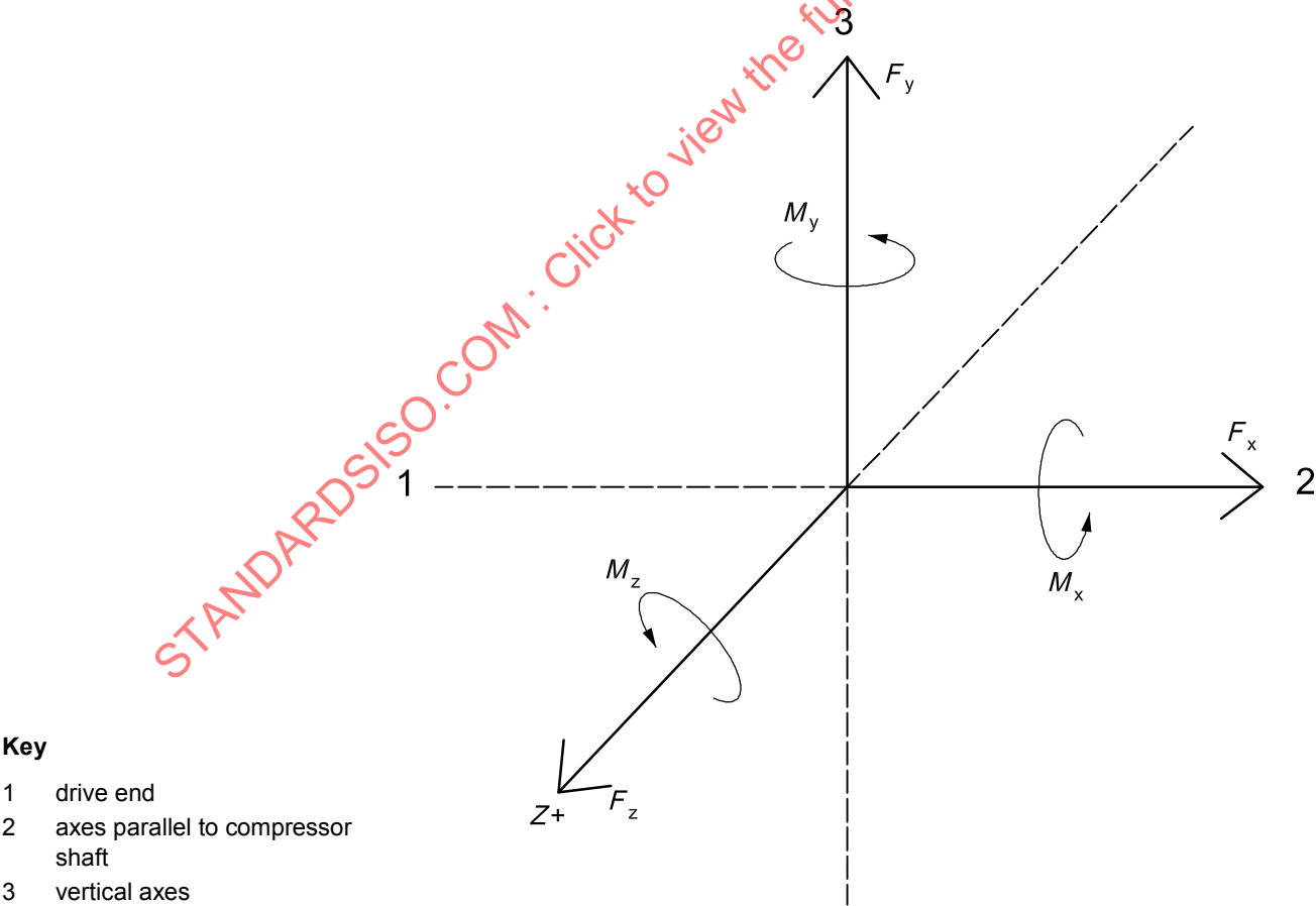
Figure C.1 — Definition of axes
