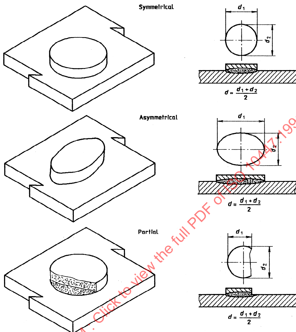
Figure 2 — Weld with plug failure
