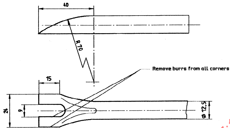
a) Chisels for weld diameter \leq 8 mm
