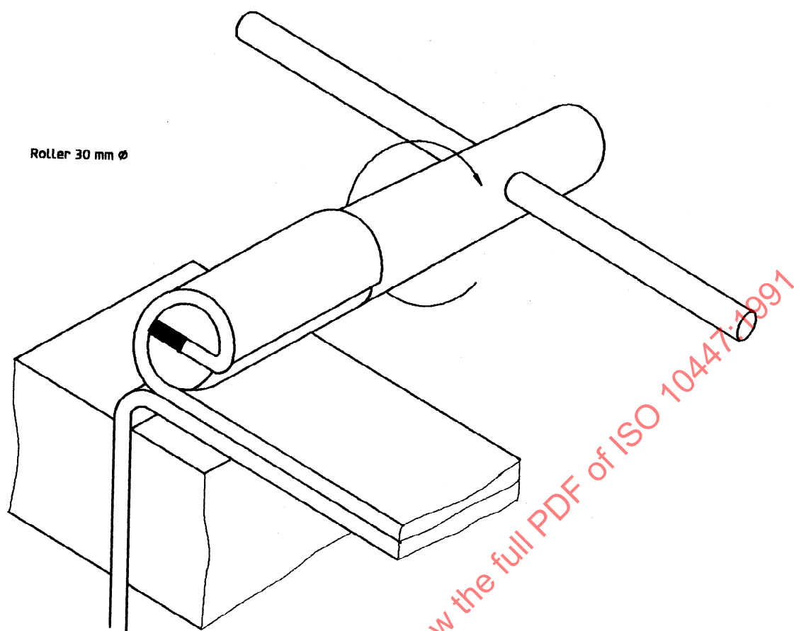
Figure 5 — Roller for manual peel test; material thickness up to 1 mm
