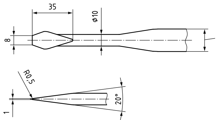
a) Type 2-1 chisel (for thickness \leq 2 mm)
