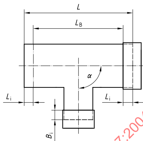
b) Unequal tee branch
