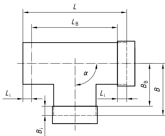
a) Equal tee branch
