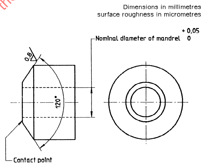
Figure 1 — Conical washer
