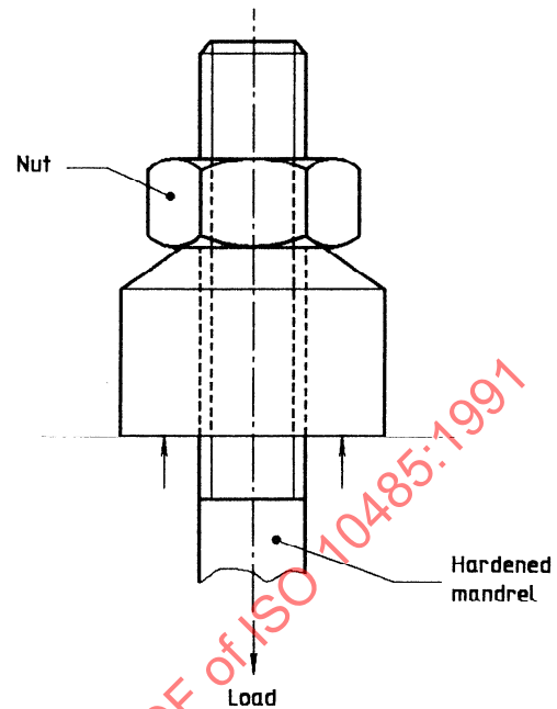
Figure 2 — Test assembly
