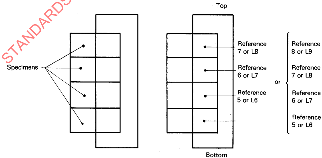
Figure 2 — Mounting for method 2
