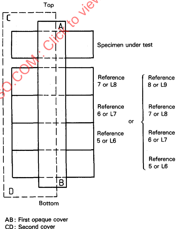
Figure 1 — Mounting for method 1
