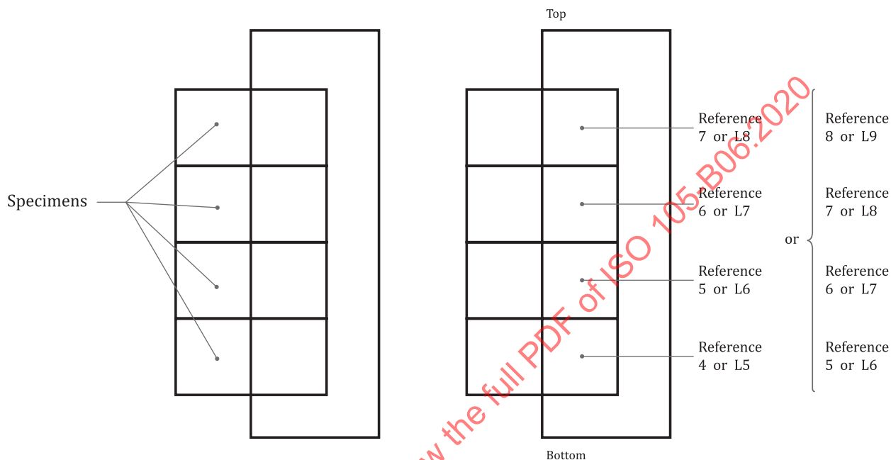
Figure 1 — Mounting for exposure method 2
