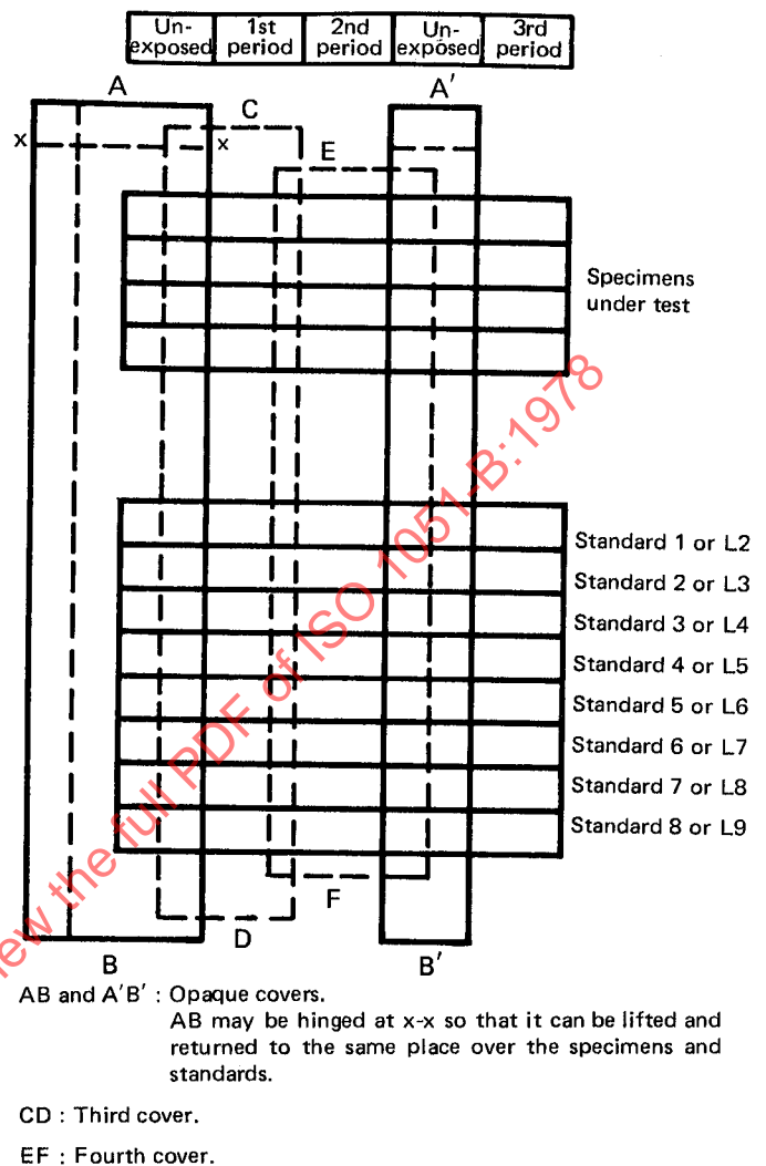
FIGURE 2 — Mounting for method 2
