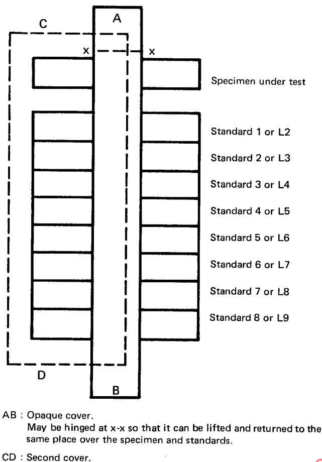
FIGURE 1 — Mounting for method 1
